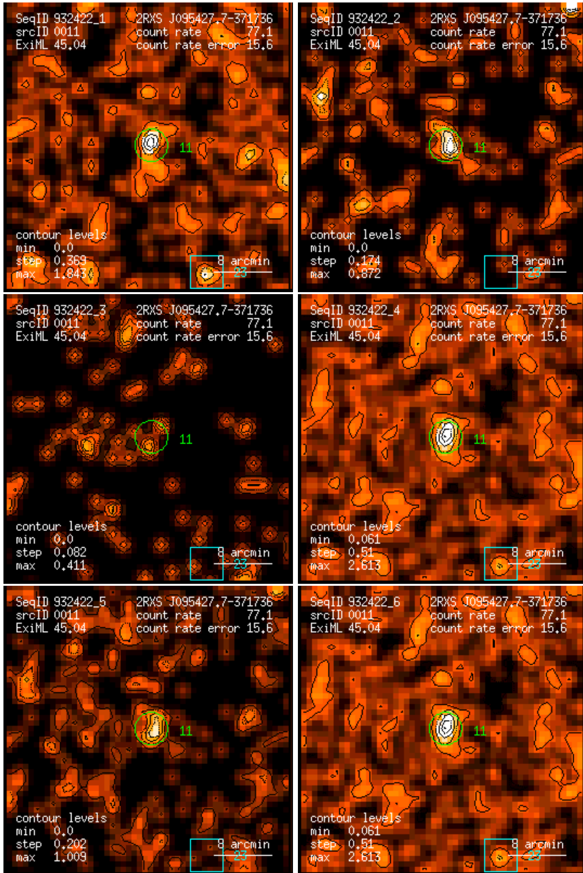
Figure 11: RASS 932422: detection 0011: band rate images, Gaussian filter: (1) PSPC channels 11 – 41, (2) 52 – 90, (3) 91 – 201, (4) 11 – 235, (5) 52 – 201, (6) 11 – 201. Broad band rates in counts/ks. Band rate contour levels in counts/ks/arcmin 2 .
