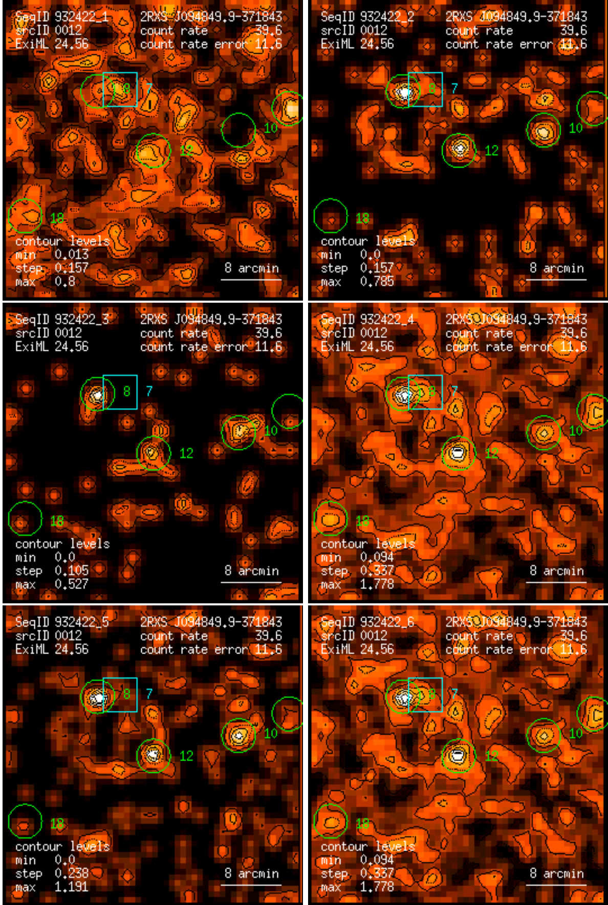
Figure 12: RASS 932422: detection 0012: band rate images, Gaussian filter: (1) PSPC channels 11 – 41, (2) 52 – 90, (3) 91 – 201, (4) 11 – 235, (5) 52 – 201, (6) 11 – 201. Broad band rates in counts/ks. Band rate contour levels in counts/ks/arcmin 2 .
