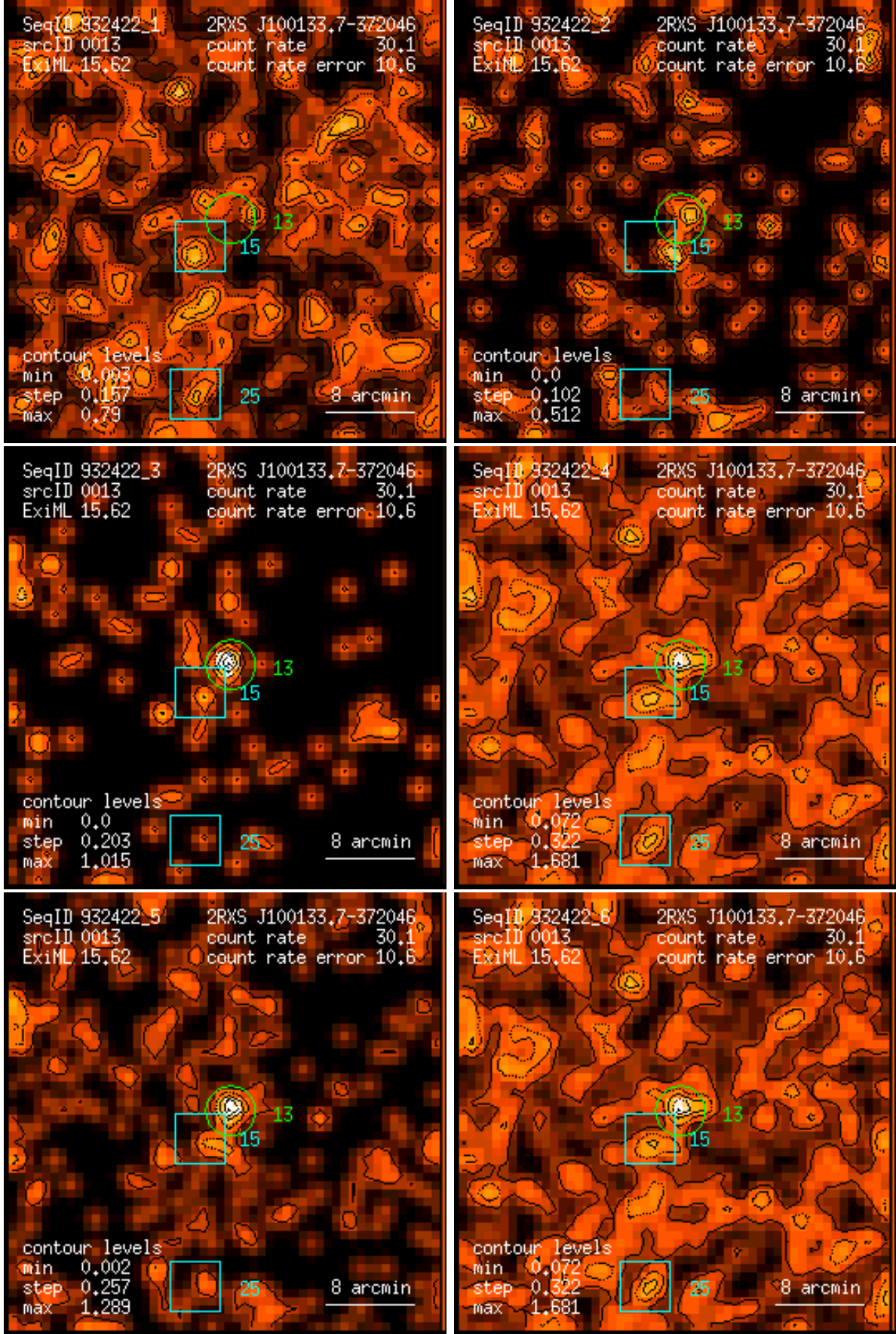
Figure 13: RASS 932422: detection 0013: band rate images, Gaussian filter: (1) PSPC channels 11 – 41, (2) 52 – 90, (3) 91 – 201, (4) 11 – 235, (5) 52 – 201, (6) 11 – 201. Broad band rates in counts/ks. Band rate contour levels in counts/ks/arcmin 2 .
