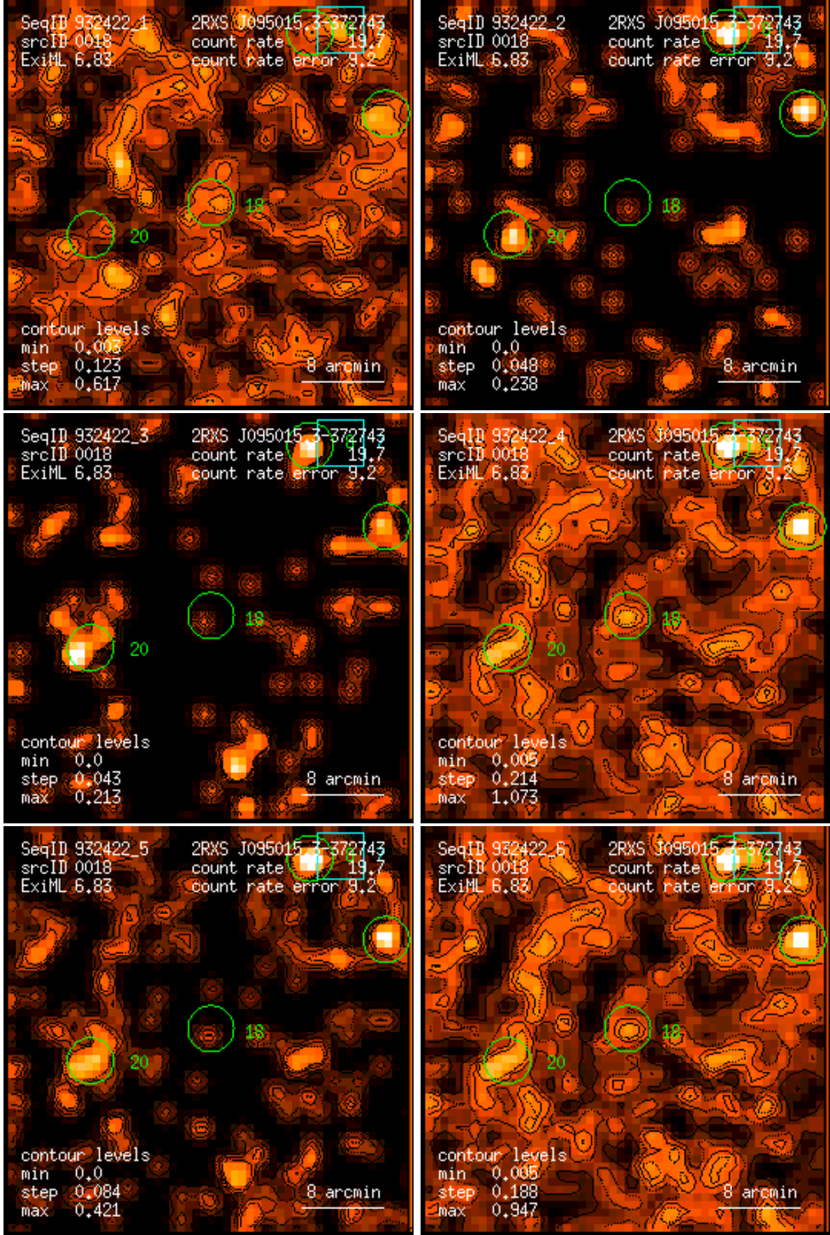
Figure 18: RASS 932422: detection 0018: band rate images, Gaussian filter: (1) PSPC channels 11 – 41, (2) 52 – 90, (3) 91 – 201, (4) 11 – 235, (5) 52 – 201, (6) 11 – 201. Broad band rates in counts/ks. Band rate contour levels in counts/ks/arcmin 2 .
