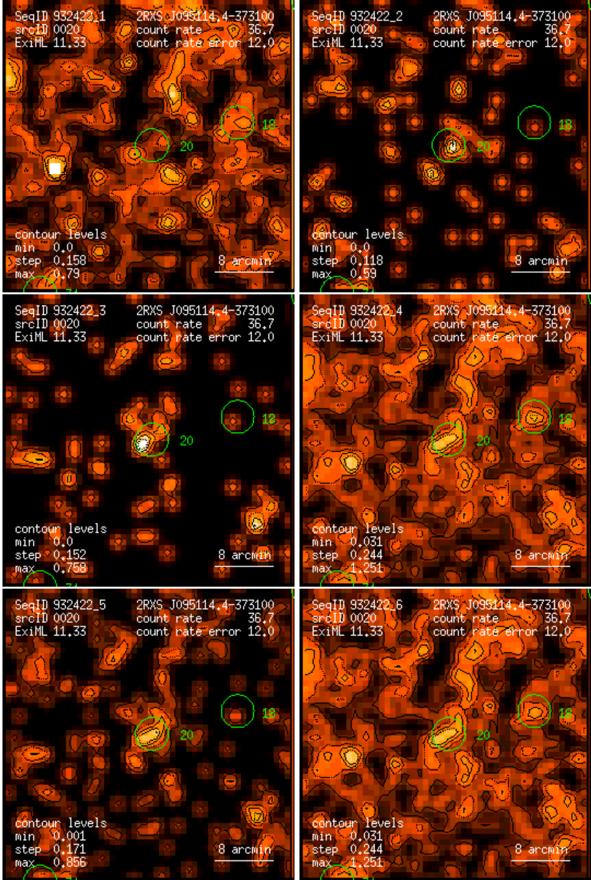
Figure 20: RASS 932422: detection 0020: band rate images, Gaussian filter: (1) PSPC channels 11 – 41, (2) 52 – 90, (3) 91 – 201, (4) 11 – 235, (5) 52 – 201, (6) 11 – 201. Broad band rates in counts/ks. Band rate contour levels in counts/ks/arcmin 2 .
