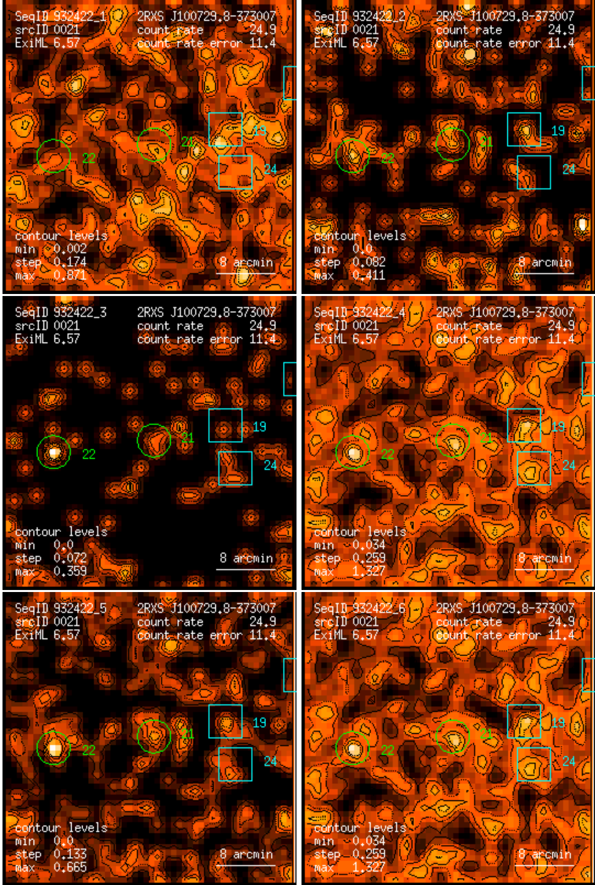
Figure 21: RASS 932422: detection 0021: band rate images, Gaussian filter: (1) PSPC channels 11 – 41, (2) 52 – 90, (3) 91 – 201, (4) 11 – 235, (5) 52 – 201, (6) 11 – 201. Broad band rates in counts/ks. Band rate contour levels in counts/ks/arcmin 2 .
