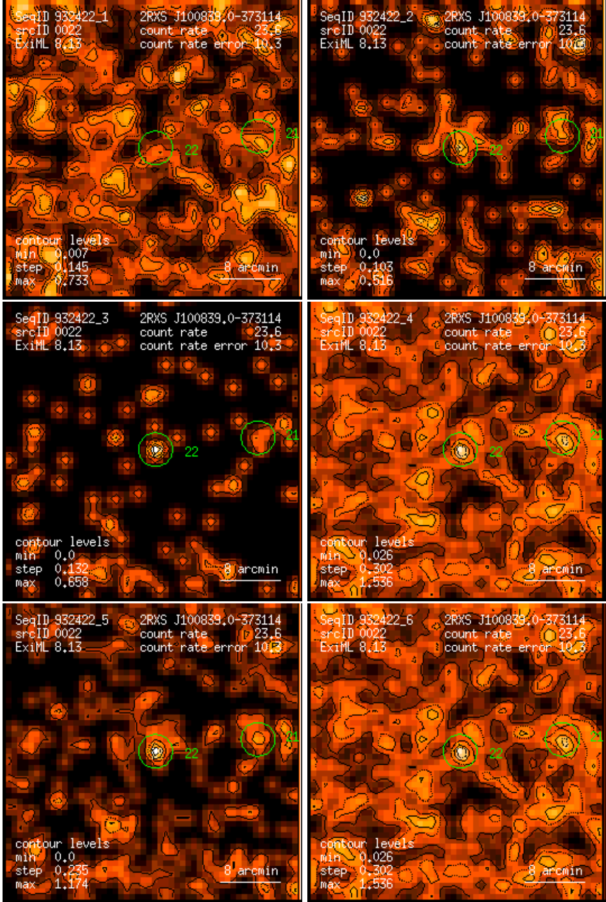
Figure 22: RASS 932422: detection 0022: band rate images, Gaussian filter: (1) PSPC channels 11 – 41, (2) 52 – 90, (3) 91 – 201, (4) 11 – 235, (5) 52 – 201, (6) 11 – 201. Broad band rates in counts/ks. Band rate contour levels in counts/ks/arcmin 2 .
