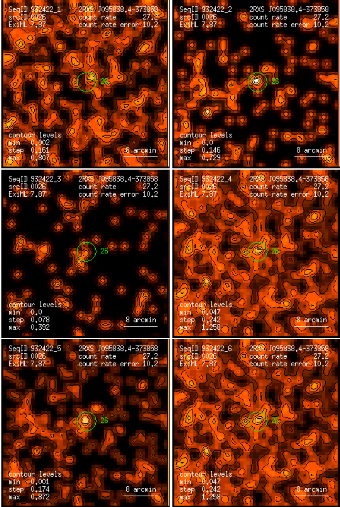
Figure 26: RASS 932422: detection 0026: band rate images, Gaussian filter: (1) PSPC channels 11 – 41, (2) 52 – 90, (3) 91 – 201, (4) 11 – 235, (5) 52 – 201, (6) 11 – 201. Broad band rates in counts/ks. Band rate contour levels in counts/ks/arcmin 2 .
