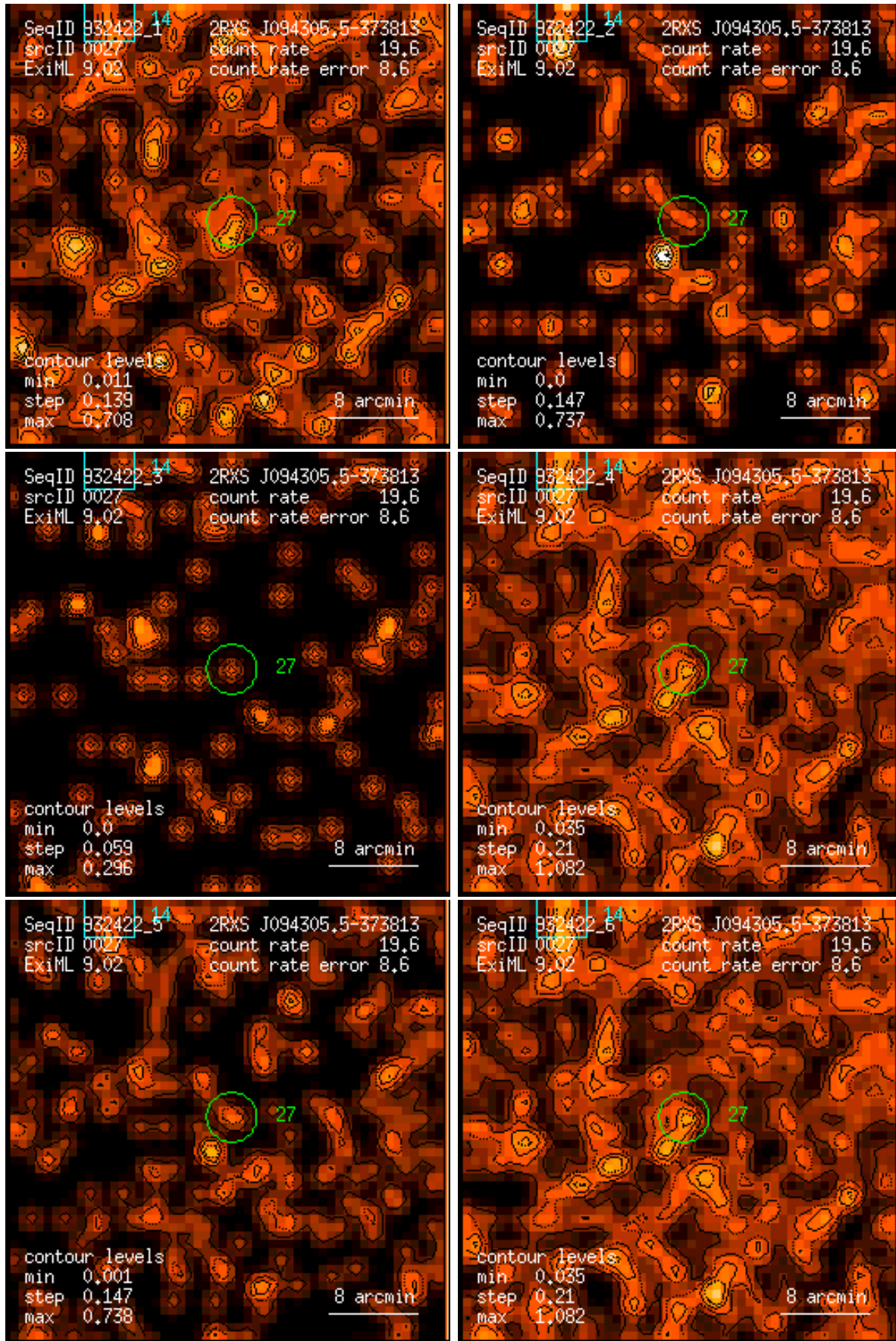
Figure 27: RASS 932422: detection 0027: band rate images, Gaussian filter: (1) PSPC channels 11 – 41, (2) 52 – 90, (3) 91 – 201, (4) 11 – 235, (5) 52 – 201, (6) 11 – 201. Broad band rates in counts/ks. Band rate contour levels in counts/ks/arcmin 2 .
