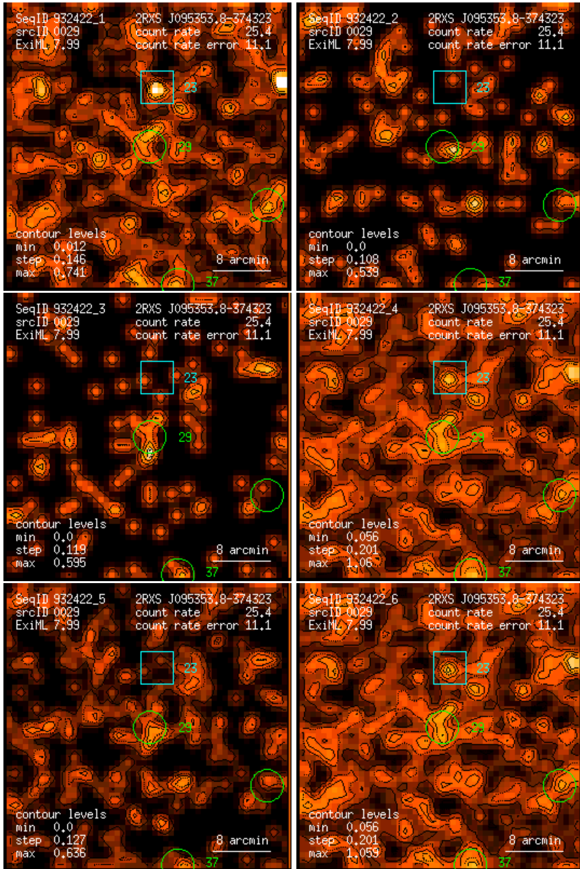
Figure 29: RASS 932422: detection 0029: band rate images, Gaussian filter: (1) PSPC channels 11 – 41, (2) 52 – 90, (3) 91 – 201, (4) 11 – 235, (5) 52 – 201, (6) 11 – 201. Broad band rates in counts/ks. Band rate contour levels in counts/ks/arcmin 2 .
