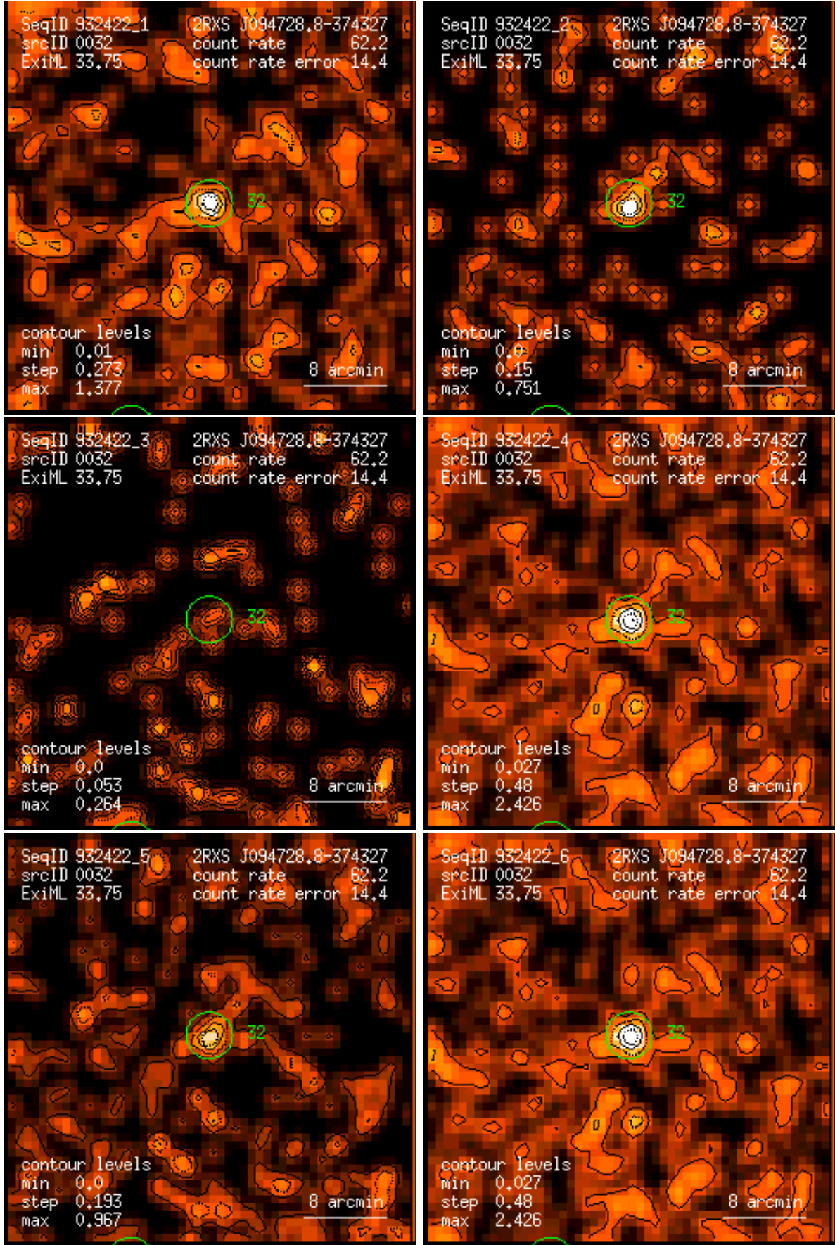
Figure 32: RASS 932422: detection 0032: band rate images, Gaussian filter: (1) PSPC channels 11 – 41, (2) 52 – 90, (3) 91 – 201, (4) 11 – 235, (5) 52 – 201, (6) 11 – 201. Broad band rates in counts/ks. Band rate contour levels in counts/ks/arcmin 2 .
