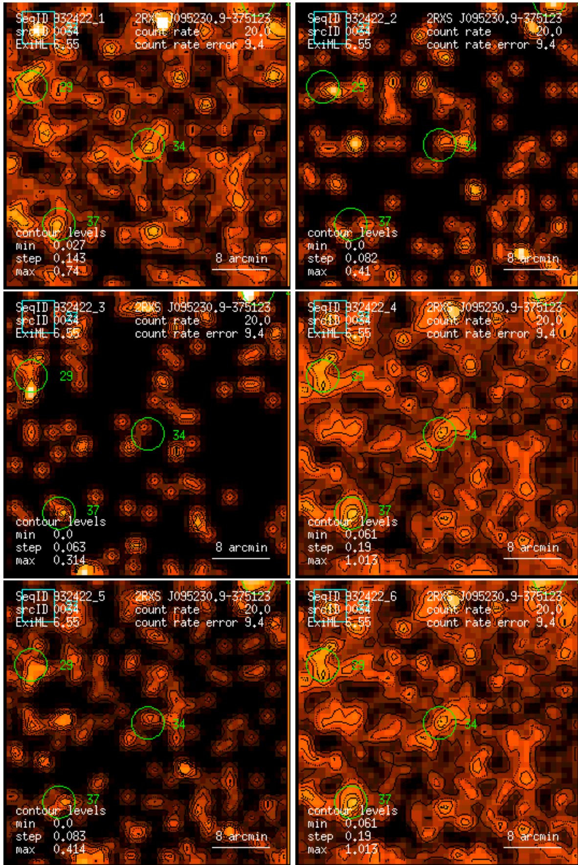
Figure 34: RASS 932422: detection 0034: band rate images, Gaussian filter: (1) PSPC channels 11 – 41, (2) 52 – 90, (3) 91 – 201, (4) 11 – 235, (5) 52 – 201, (6) 11 – 201. Broad band rates in counts/ks. Band rate contour levels in counts/ks/arcmin 2 .
