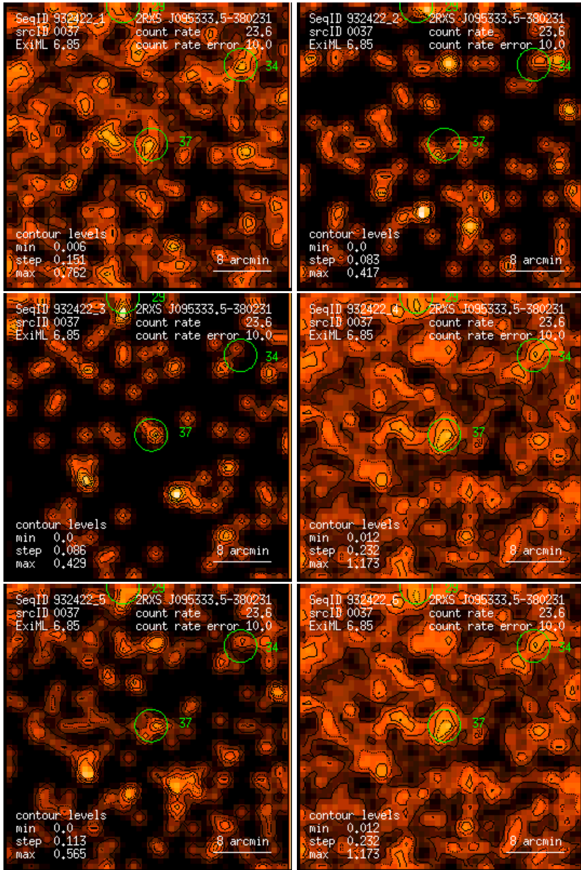
Figure 37: RASS 932422: detection 0037: band rate images, Gaussian filter: (1) PSPC channels 11 – 41, (2) 52 – 90, (3) 91 – 201, (4) 11 – 235, (5) 52 – 201, (6) 11 – 201. Broad band rates in counts/ks. Band rate contour levels in counts/ks/arcmin 2 .
