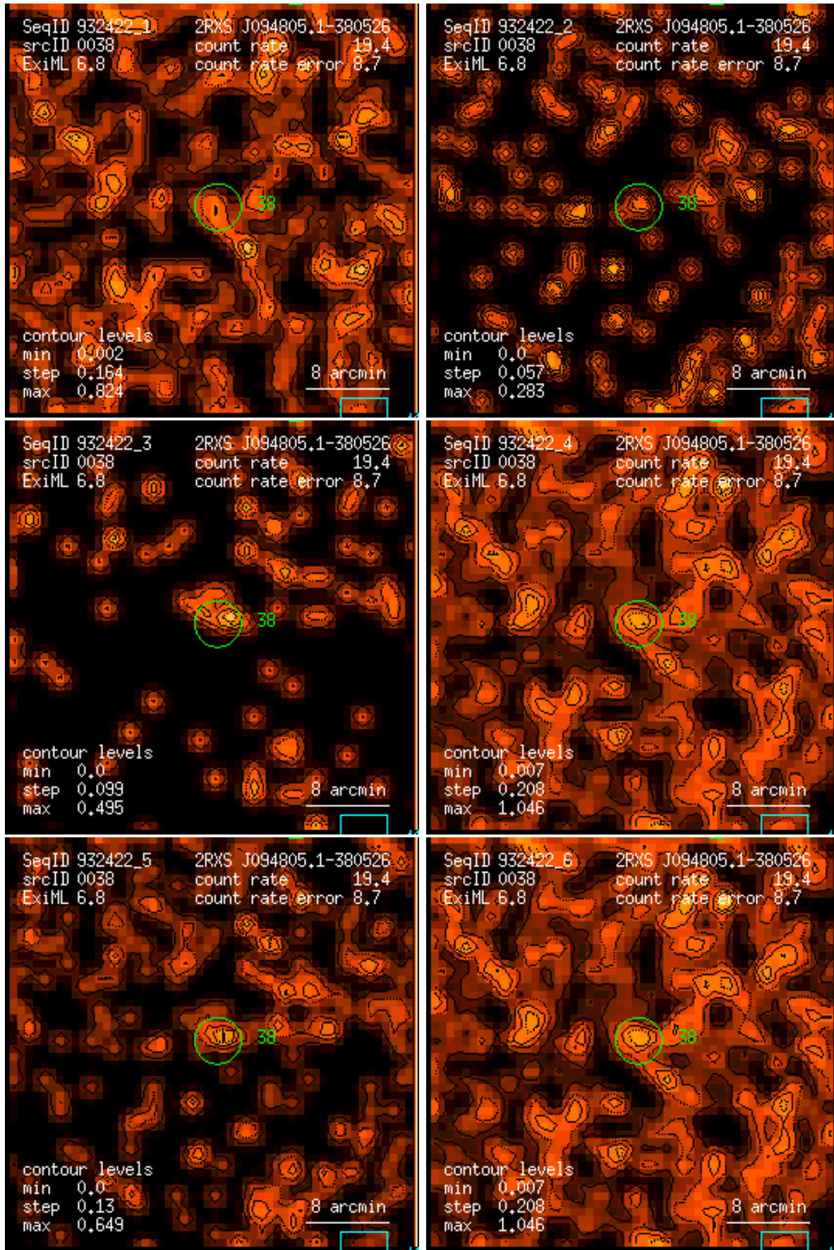
Figure 38: RASS 932422: detection 0038: band rate images, Gaussian filter: (1) PSPC channels 11 – 41, (2) 52 – 90, (3) 91 – 201, (4) 11 – 235, (5) 52 – 201, (6) 11 – 201. Broad band rates in counts/ks. Band rate contour levels in counts/ks/arcmin 2 .
