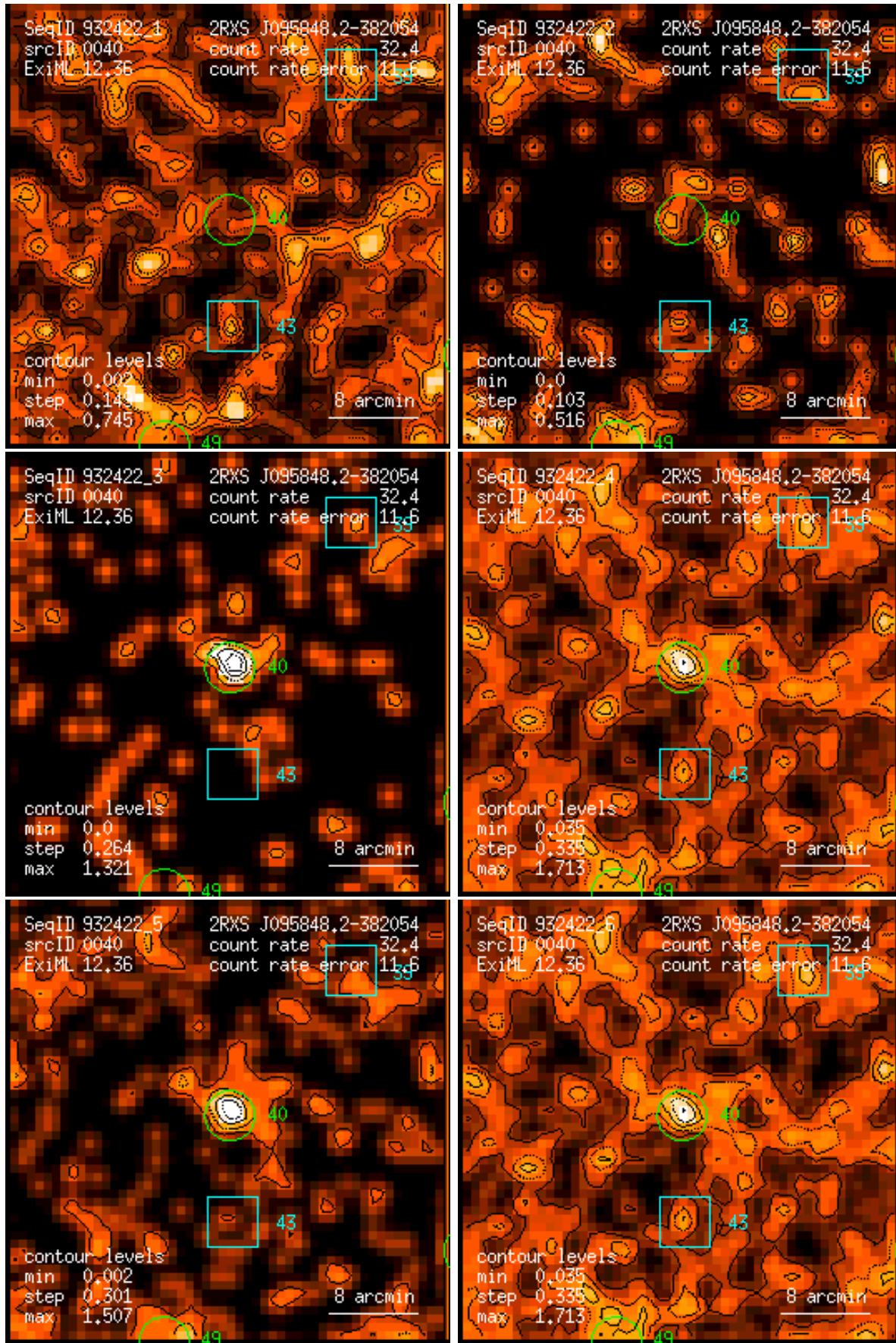
Figure 40: RASS 932422: detection 0040: band rate images, Gaussian filter: (1) PSPC channels 11 – 41, (2) 52 – 90, (3) 91 – 201, (4) 11 – 235, (5) 52 – 201, (6) 11 – 201. Broad band rates in counts/ks. Band rate contour levels in counts/ks/arcmin 2 .
