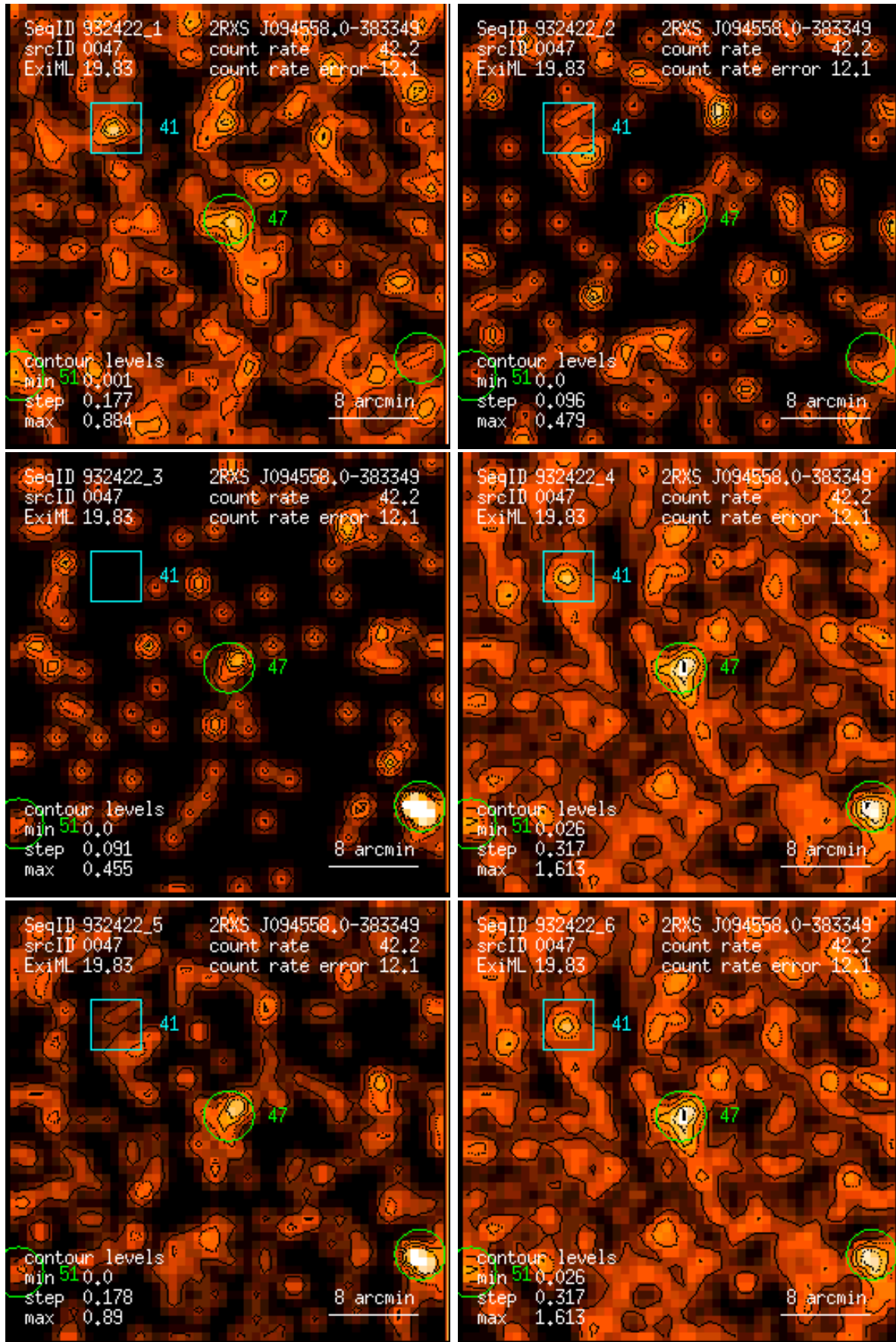
Figure 47: RASS 932422: detection 0047: band rate images, Gaussian filter: (1) PSPC channels 11 – 41, (2) 52 – 90, (3) 91 – 201, (4) 11 – 235, (5) 52 – 201, (6) 11 – 201. Broad band rates in counts/ks. Band rate contour levels in counts/ks/arcmin 2 .
