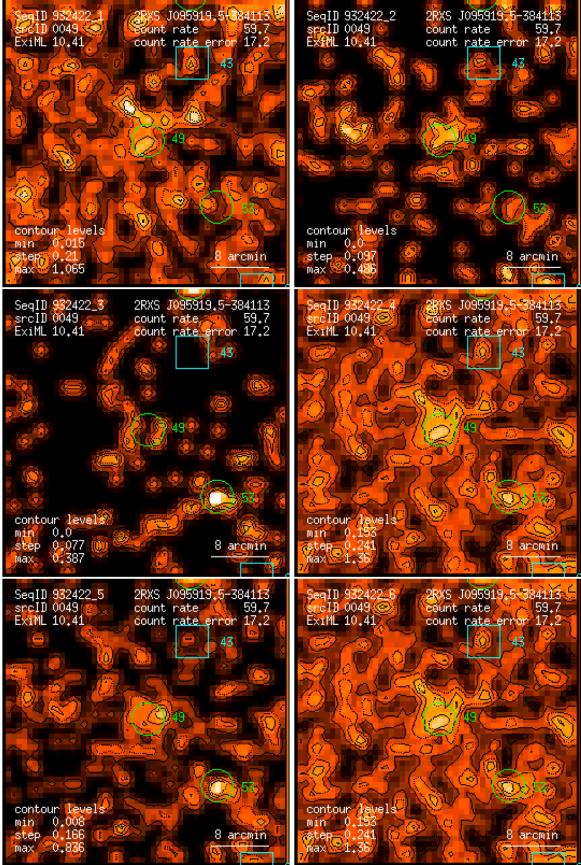
Figure 49: RASS 932422: detection 0049: band rate images, Gaussian filter: (1) PSPC channels 11 – 41, (2) 52 – 90, (3) 91 – 201, (4) 11 – 235, (5) 52 – 201, (6) 11 – 201. Broad band rates in counts/ks. Band rate contour levels in counts/ks/arcmin 2 .
