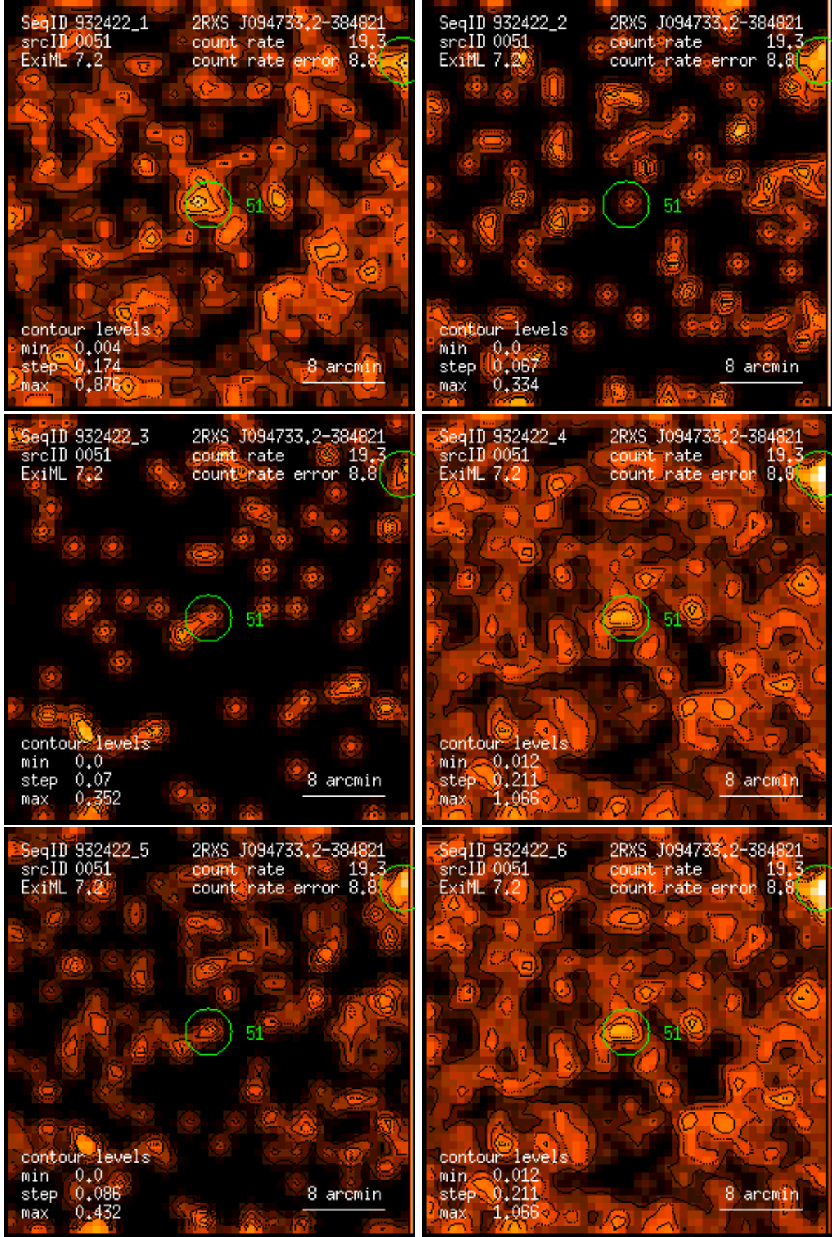
Figure 51: RASS 932422: detection 0051: band rate images, Gaussian filter: (1) PSPC channels 11 – 41, (2) 52 – 90, (3) 91 – 201, (4) 11 – 235, (5) 52 – 201, (6) 11 – 201. Broad band rates in counts/ks. Band rate contour levels in counts/ks/arcmin 2 .
