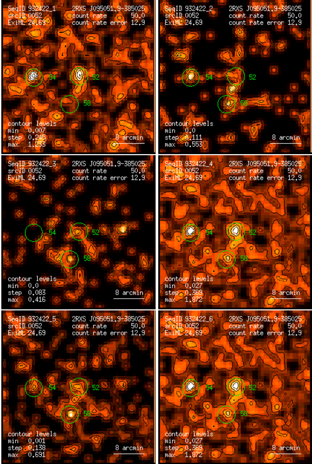
Figure 52: RASS 932422: detection 0052: band rate images, Gaussian filter: (1) PSPC channels 11 – 41, (2) 52 – 90, (3) 91 – 201, (4) 11 – 235, (5) 52 – 201, (6) 11 – 201. Broad band rates in counts/ks. Band rate contour levels in counts/ks/arcmin 2 .
