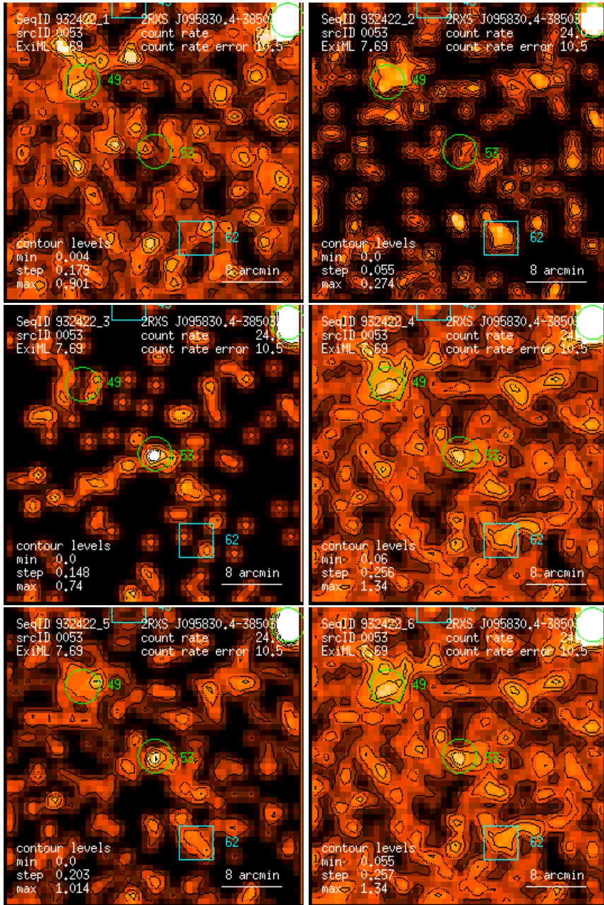
Figure 53: RASS 932422: detection 0053: band rate images, Gaussian filter: (1) PSPC channels 11 – 41, (2) 52 – 90, (3) 91 – 201, (4) 11 – 235, (5) 52 – 201, (6) 11 – 201. Broad band rates in counts/ks. Band rate contour levels in counts/ks/arcmin 2 .
