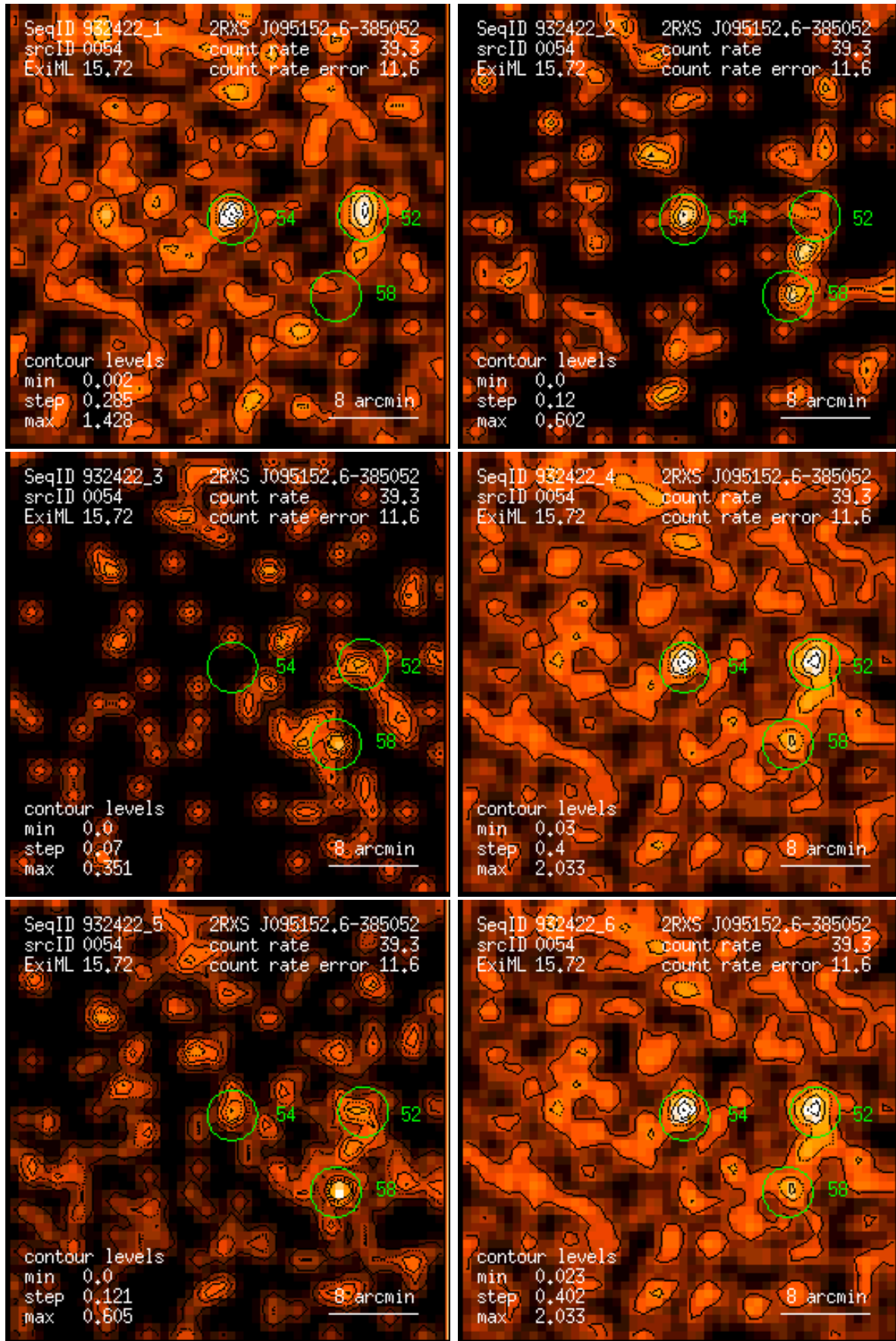
Figure 54: RASS 932422: detection 0054: band rate images, Gaussian filter: (1) PSPC channels 11 – 41, (2) 52 – 90, (3) 91 – 201, (4) 11 – 235, (5) 52 – 201, (6) 11 – 201. Broad band rates in counts/ks. Band rate contour levels in counts/ks/arcmin 2 .
