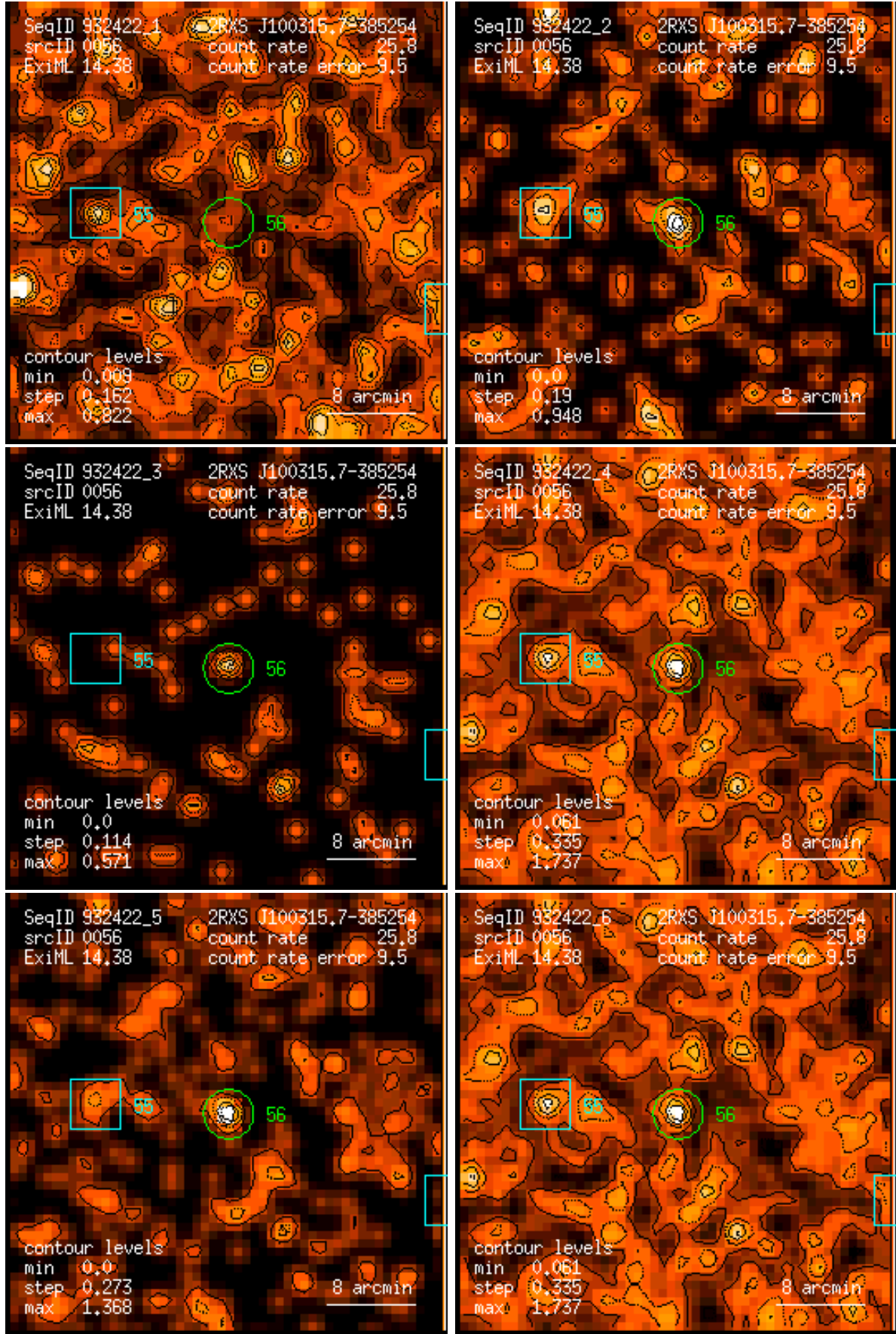
Figure 56: RASS 932422: detection 0056: band rate images, Gaussian filter: (1) PSPC channels 11 – 41, (2) 52 – 90, (3) 91 – 201, (4) 11 – 235, (5) 52 – 201, (6) 11 – 201. Broad band rates in counts/ks. Band rate contour levels in counts/ks/arcmin 2 .
