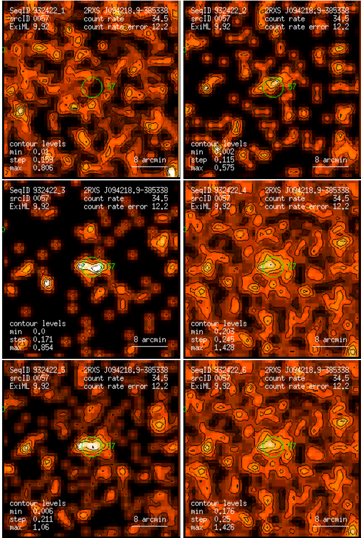
Figure 57: RASS 932422: detection 0057: band rate images, Gaussian filter: (1) PSPC channels 11 – 41, (2) 52 – 90, (3) 91 – 201, (4) 11 – 235, (5) 52 – 201, (6) 11 – 201. Broad band rates in counts/ks. Band rate contour levels in counts/ks/arcmin 2 .
