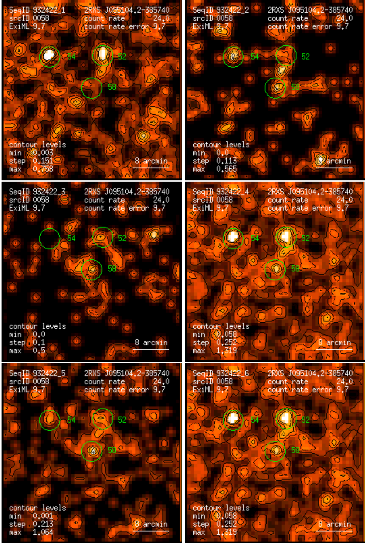
Figure 58: RASS 932422: detection 0058: band rate images, Gaussian filter: (1) PSPC channels 11 – 41, (2) 52 – 90, (3) 91 – 201, (4) 11 – 235, (5) 52 – 201, (6) 11 – 201. Broad band rates in counts/ks. Band rate contour levels in counts/ks/arcmin 2 .
