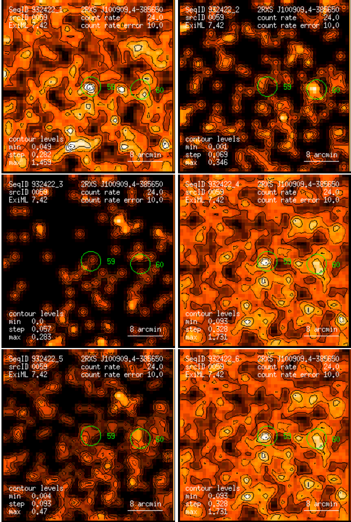
Figure 59: RASS 932422: detection 0059: band rate images, Gaussian filter: (1) PSPC channels 11 – 41, (2) 52 – 90, (3) 91 – 201, (4) 11 – 235, (5) 52 – 201, (6) 11 – 201. Broad band rates in counts/ks. Band rate contour levels in counts/ks/arcmin 2 .
