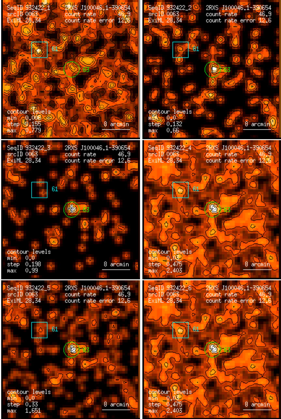
Figure 63: RASS 932422: detection 0063: band rate images, Gaussian filter: (1) PSPC channels 11 – 41, (2) 52 – 90, (3) 91 – 201, (4) 11 – 235, (5) 52 – 201, (6) 11 – 201. Broad band rates in counts/ks. Band rate contour levels in counts/ks/arcmin 2 .
