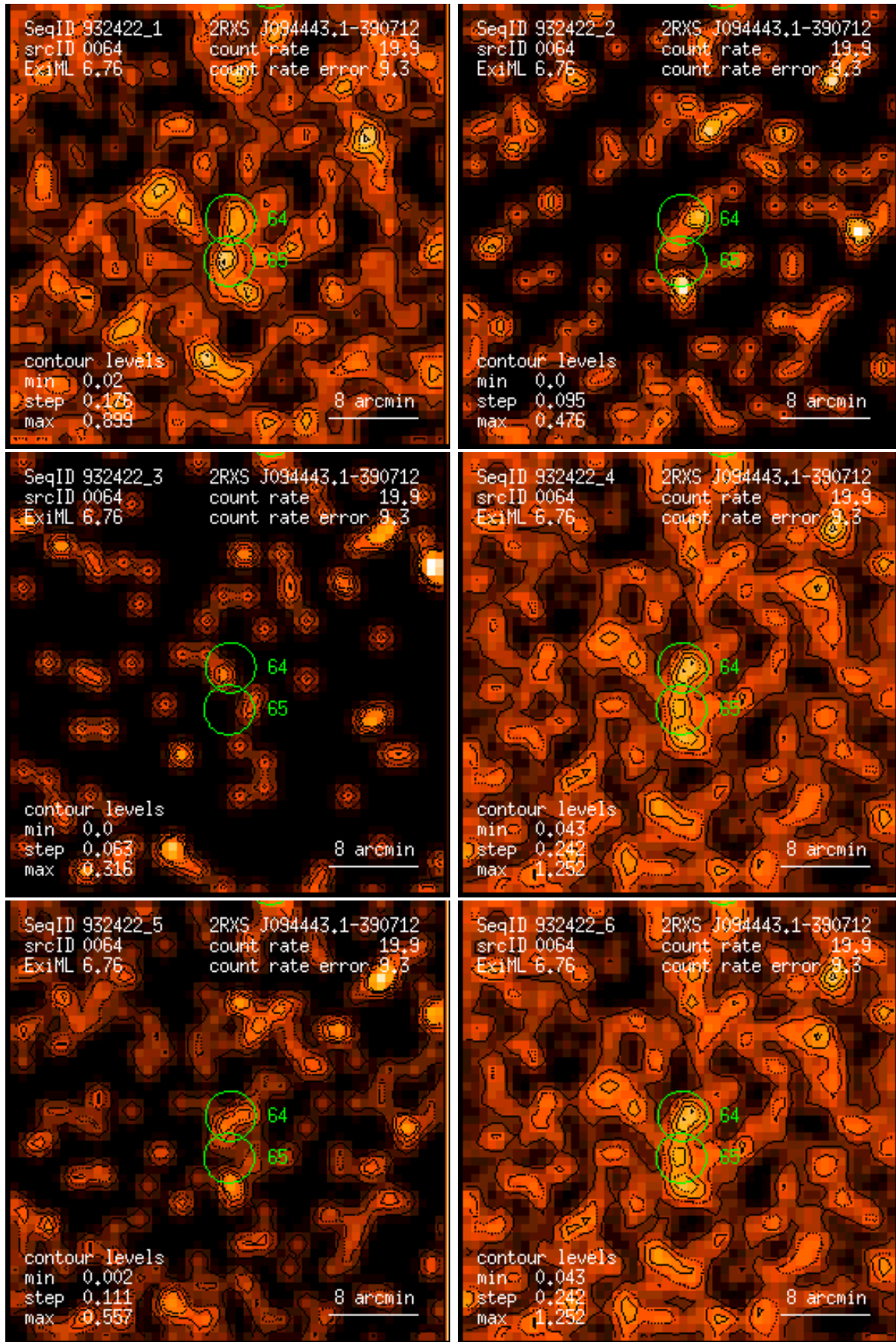
Figure 64: RASS 932422: detection 0064: band rate images, Gaussian filter: (1) PSPC channels 11 – 41, (2) 52 – 90, (3) 91 – 201, (4) 11 – 235, (5) 52 – 201, (6) 11 – 201. Broad band rates in counts/ks. Band rate contour levels in counts/ks/arcmin 2 .
