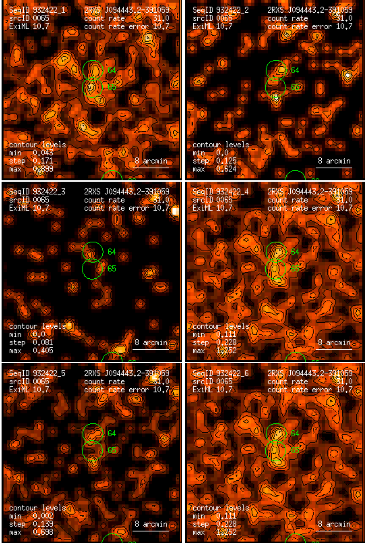
Figure 65: RASS 932422: detection 0065: band rate images, Gaussian filter: (1) PSPC channels 11 – 41, (2) 52 – 90, (3) 91 – 201, (4) 11 – 235, (5) 52 – 201, (6) 11 – 201. Broad band rates in counts/ks. Band rate contour levels in counts/ks/arcmin 2 .
