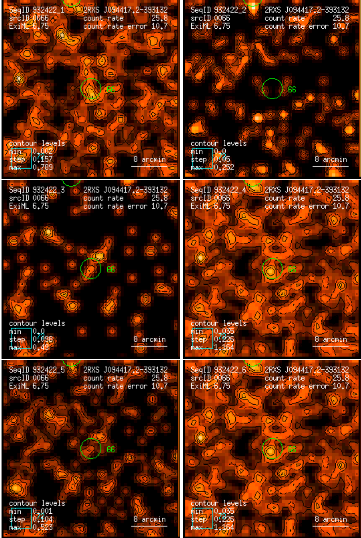
Figure 66: RASS 932422: detection 0066: band rate images, Gaussian filter: (1) PSPC channels 11 – 41, (2) 52 – 90, (3) 91 – 201, (4) 11 – 235, (5) 52 – 201, (6) 11 – 201. Broad band rates in counts/ks. Band rate contour levels in counts/ks/arcmin 2 .
