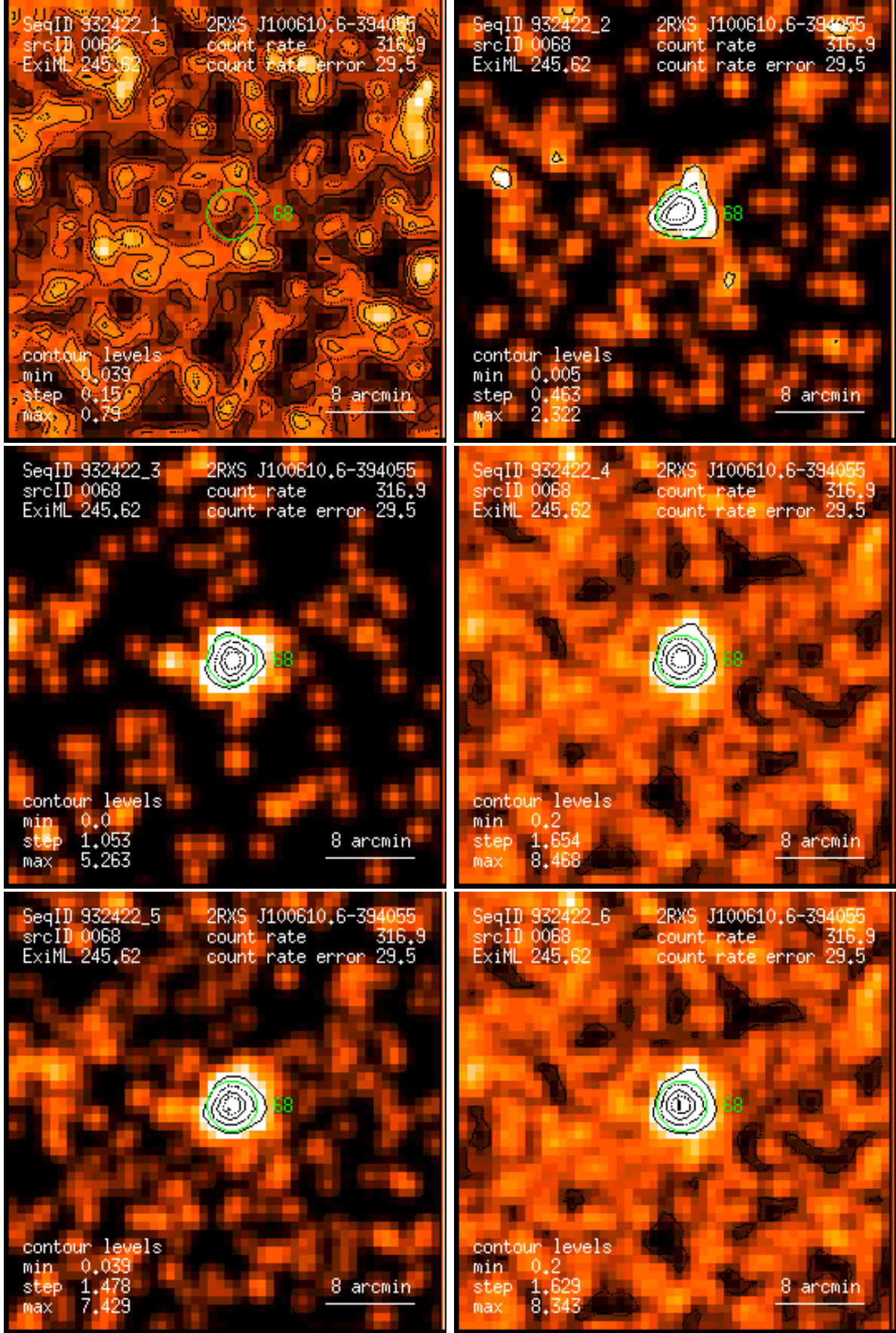
Figure 68: RASS 932422: detection 0068: band rate images, Gaussian filter: (1) PSPC channels 11 – 41, (2) 52 – 90, (3) 91 – 201, (4) 11 – 235, (5) 52 – 201, (6) 11 – 201. Broad band rates in counts/ks. Band rate contour levels in counts/ks/arcmin 2 .
