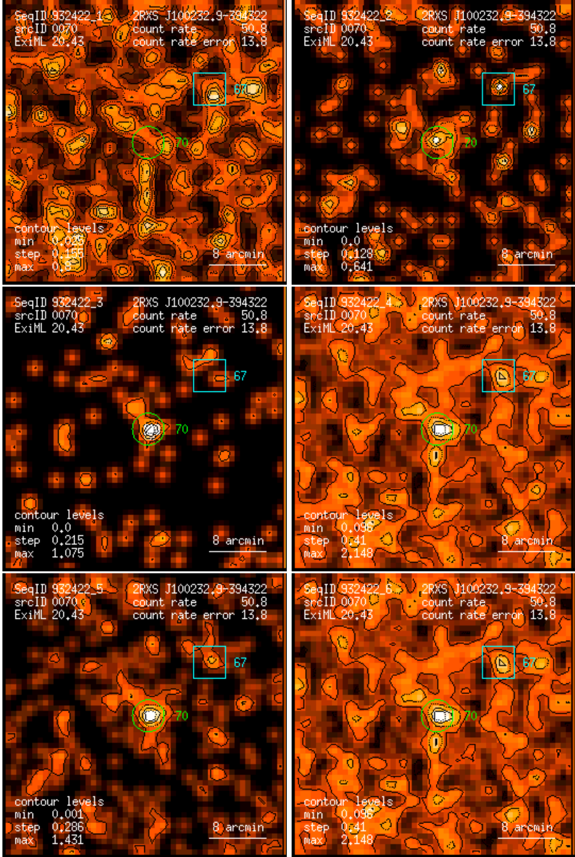
Figure 70: RASS 932422: detection 0070: band rate images, Gaussian filter: (1) PSPC channels 11 – 41, (2) 52 – 90, (3) 91 – 201, (4) 11 – 235, (5) 52 – 201, (6) 11 – 201. Broad band rates in counts/ks. Band rate contour levels in counts/ks/arcmin 2 .
