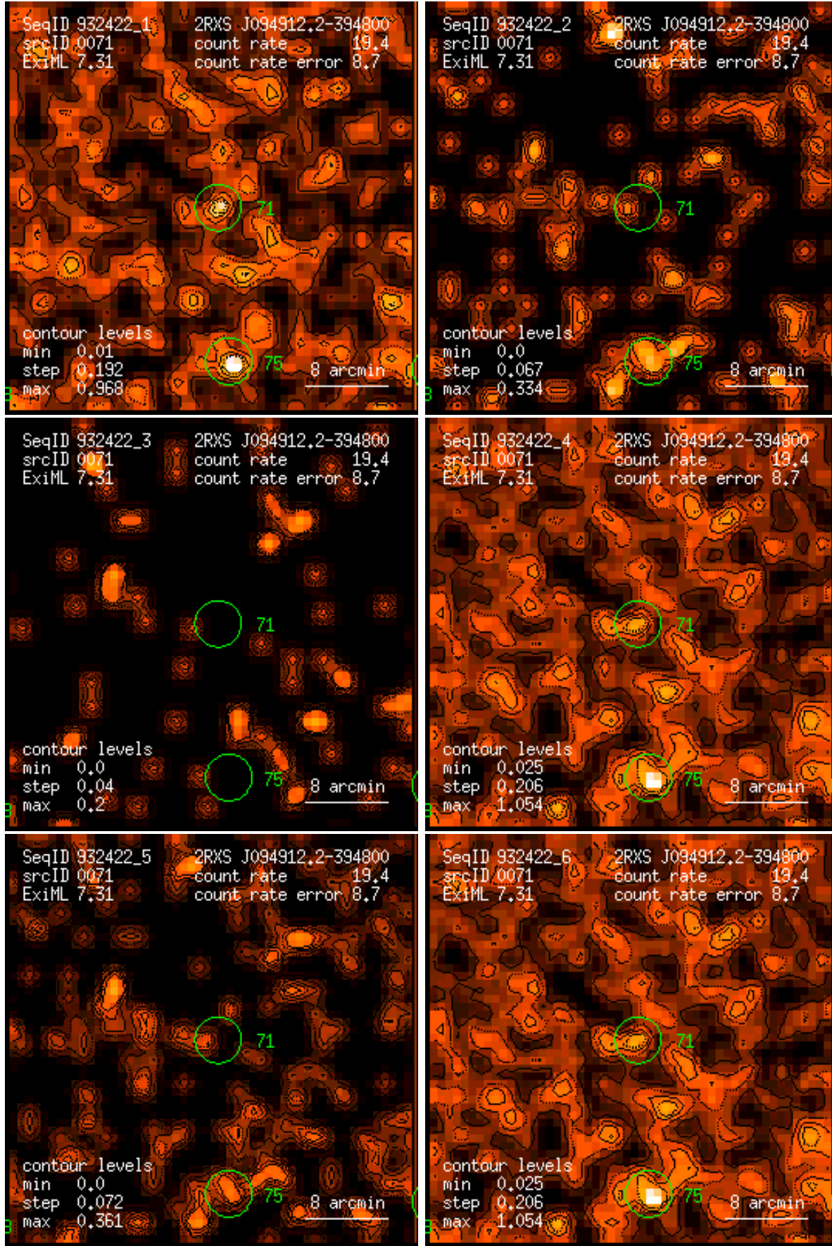
Figure 71: RASS 932422: detection 0071: band rate images, Gaussian filter: (1) PSPC channels 11 – 41, (2) 52 – 90, (3) 91 – 201, (4) 11 – 235, (5) 52 – 201, (6) 11 – 201. Broad band rates in counts/ks. Band rate contour levels in counts/ks/arcmin 2 .
