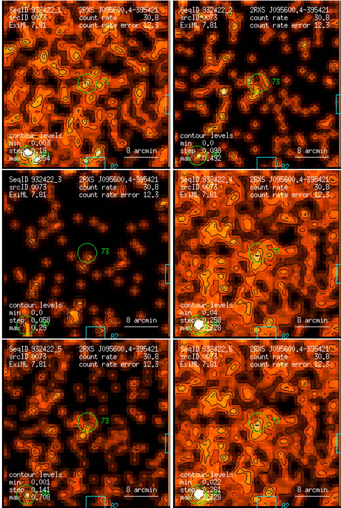
Figure 73: RASS 932422: detection 0073: band rate images, Gaussian filter: (1) PSPC channels 11 – 41, (2) 52 – 90, (3) 91 – 201, (4) 11 – 235, (5) 52 – 201, (6) 11 – 201. Broad band rates in counts/ks. Band rate contour levels in counts/ks/arcmin 2 .
