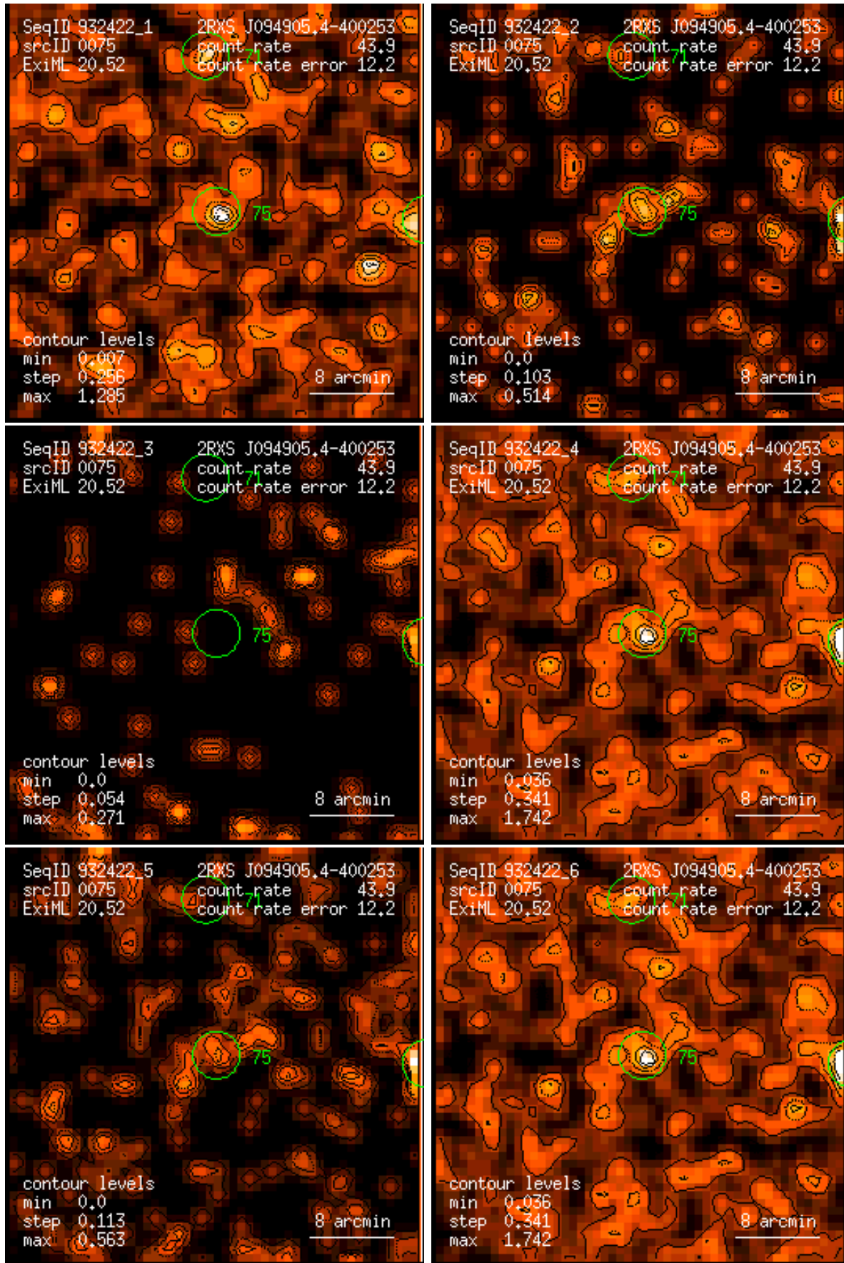
Figure 75: RASS 932422: detection 0075: band rate images, Gaussian filter: (1) PSPC channels 11 – 41, (2) 52 – 90, (3) 91 – 201, (4) 11 – 235, (5) 52 – 201, (6) 11 – 201. Broad band rates in counts/ks. Band rate contour levels in counts/ks/arcmin 2 .
