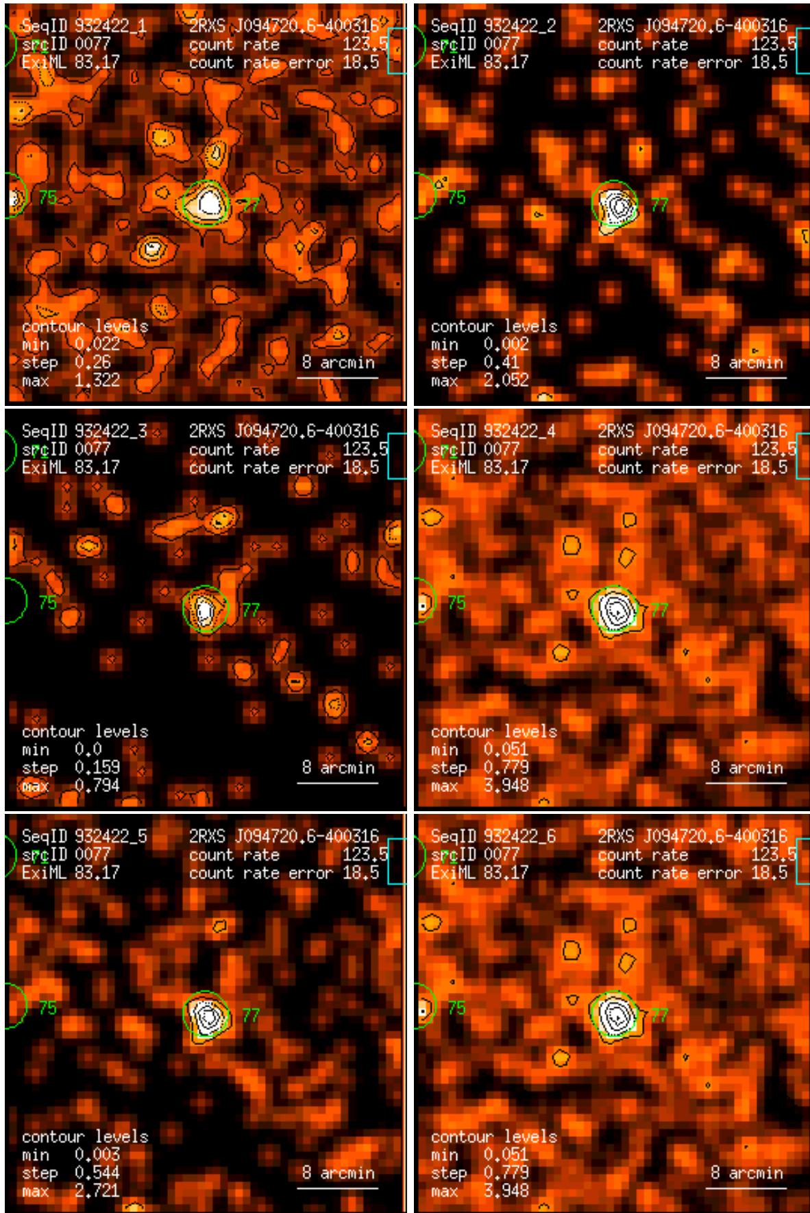
Figure 77: RASS 932422: detection 0077: band rate images, Gaussian filter: (1) PSPC channels 11 – 41, (2) 52 – 90, (3) 91 – 201, (4) 11 – 235, (5) 52 – 201, (6) 11 – 201. Broad band rates in counts/ks. Band rate contour levels in counts/ks/arcmin 2 .
