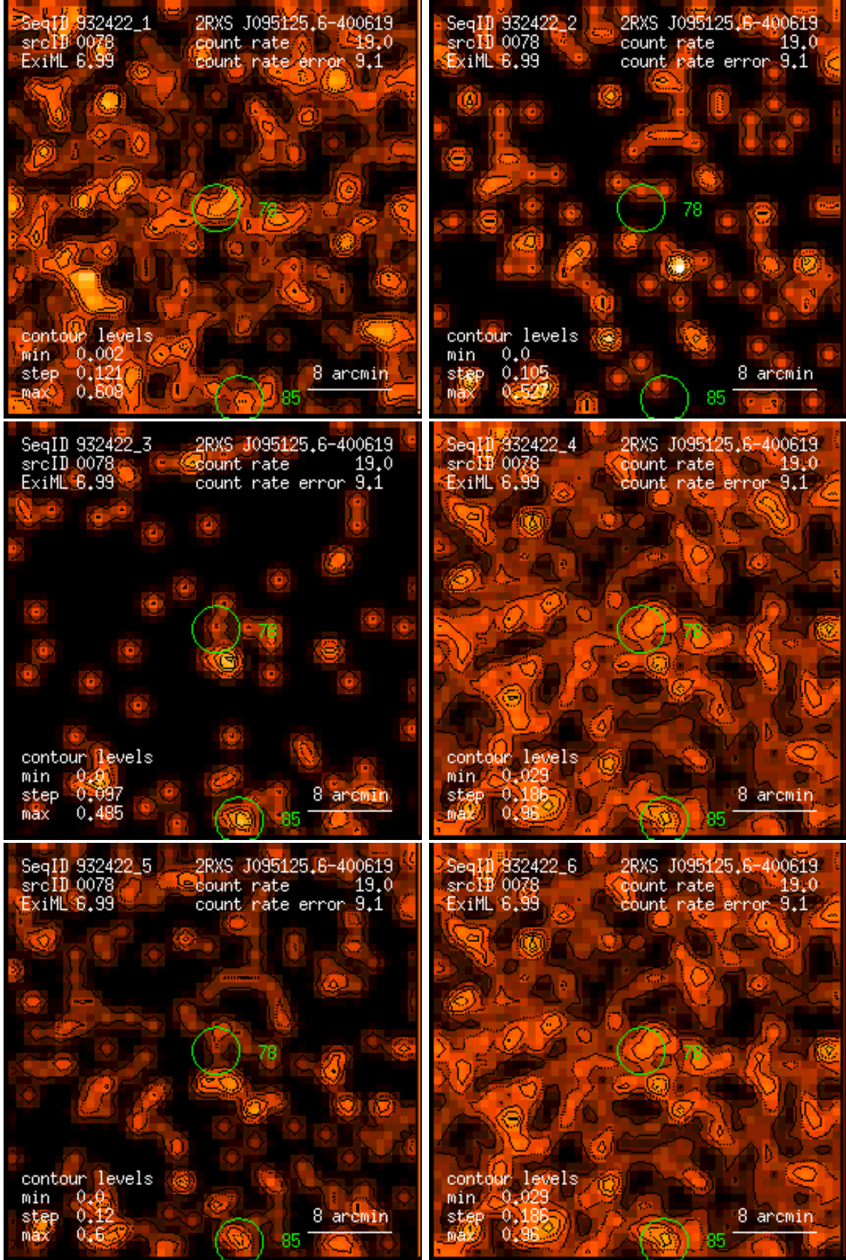
Figure 78: RASS 932422: detection 0078: band rate images, Gaussian filter: (1) PSPC channels 11 – 41, (2) 52 – 90, (3) 91 – 201, (4) 11 – 235, (5) 52 – 201, (6) 11 – 201. Broad band rates in counts/ks. Band rate contour levels in counts/ks/arcmin 2 .
