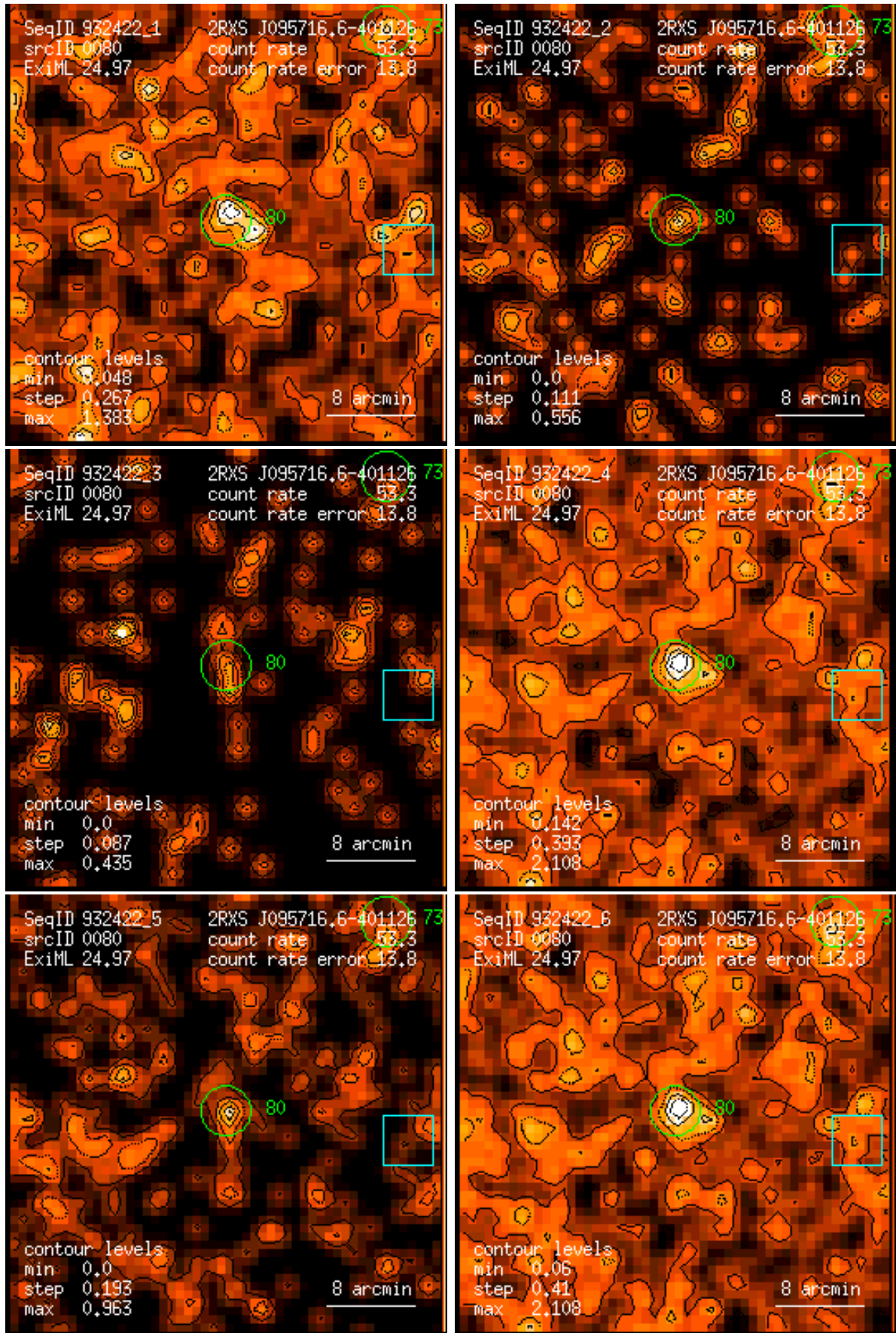
Figure 80: RASS 932422: detection 0080: band rate images, Gaussian filter: (1) PSPC channels 11 – 41, (2) 52 – 90, (3) 91 – 201, (4) 11 – 235, (5) 52 – 201, (6) 11 – 201. Broad band rates in counts/ks. Band rate contour levels in counts/ks/arcmin 2 .
