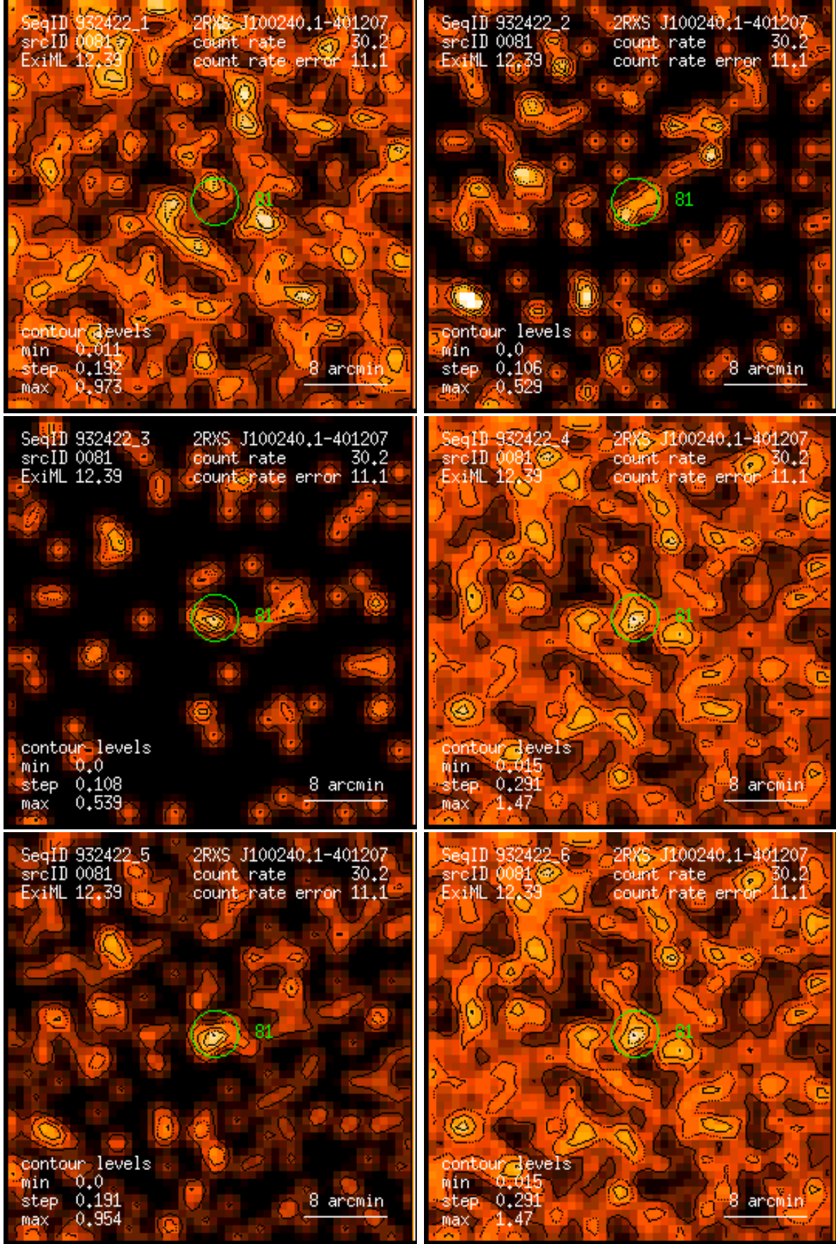
Figure 81: RASS 932422: detection 0081: band rate images, Gaussian filter: (1) PSPC channels 11 – 41, (2) 52 – 90, (3) 91 – 201, (4) 11 – 235, (5) 52 – 201, (6) 11 – 201. Broad band rates in counts/ks. Band rate contour levels in counts/ks/arcmin 2 .
