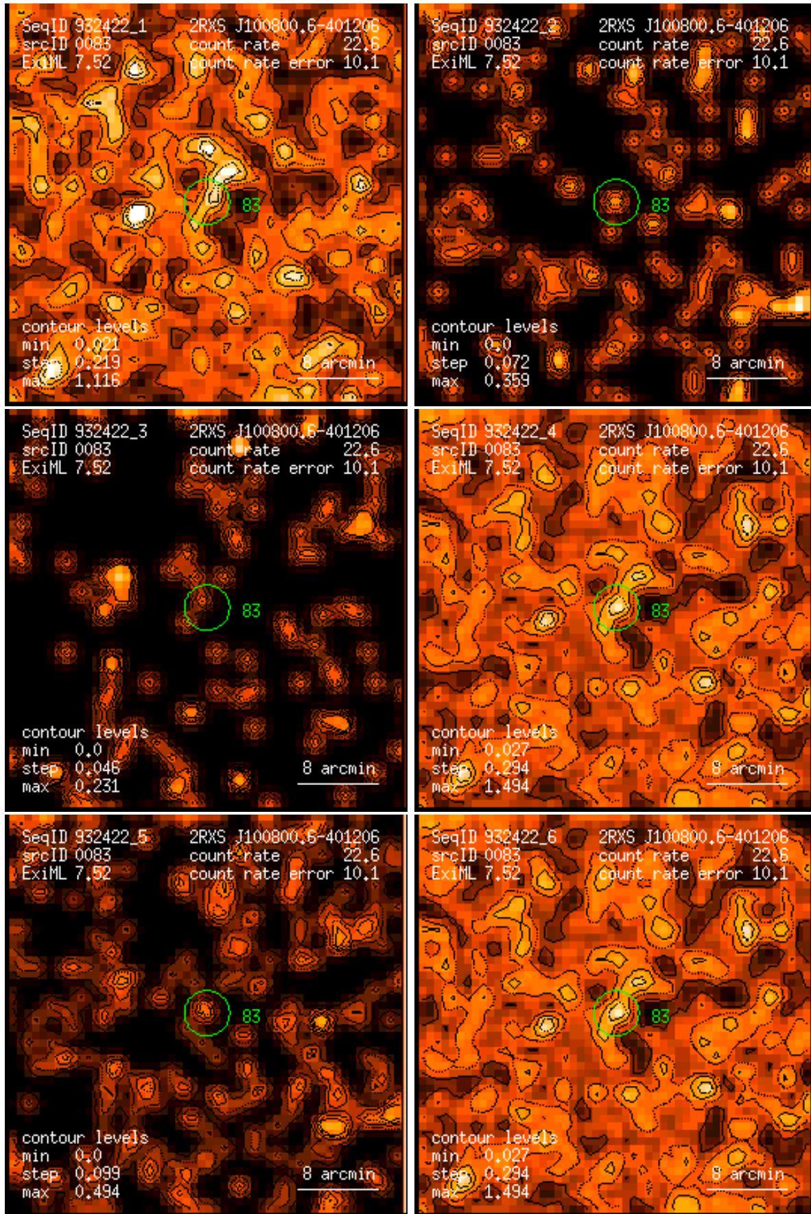
Figure 83: RASS 932422: detection 0083: band rate images, Gaussian filter: (1) PSPC channels 11 – 41, (2) 52 – 90, (3) 91 – 201, (4) 11 – 235, (5) 52 – 201, (6) 11 – 201. Broad band rates in counts/ks. Band rate contour levels in counts/ks/arcmin 2 .
