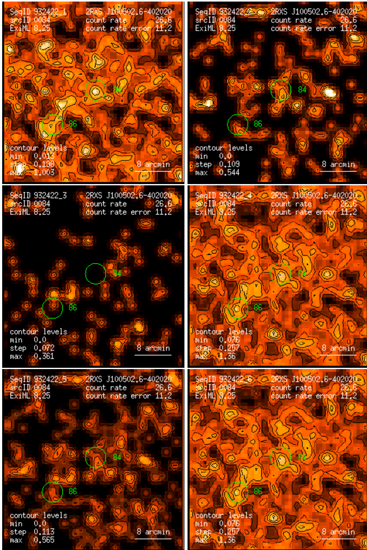
Figure 84: RASS 932422: detection 0084: band rate images, Gaussian filter: (1) PSPC channels 11 – 41, (2) 52 – 90, (3) 91 – 201, (4) 11 – 235, (5) 52 – 201, (6) 11 – 201. Broad band rates in counts/ks. Band rate contour levels in counts/ks/arcmin 2 .
