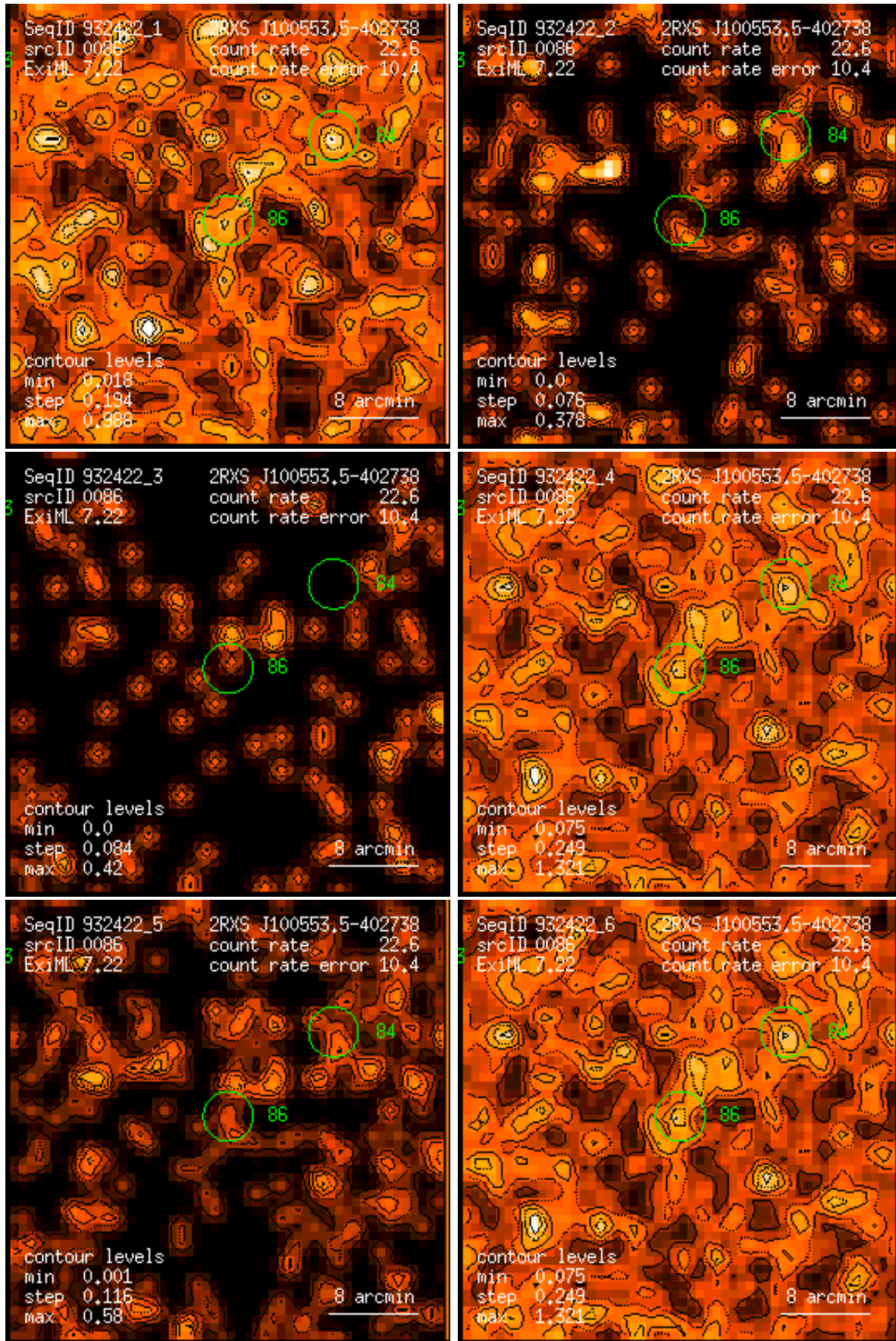
Figure 86: RASS 932422: detection 0086: band rate images, Gaussian filter: (1) PSPC channels 11 – 41, (2) 52 – 90, (3) 91 – 201, (4) 11 – 235, (5) 52 – 201, (6) 11 – 201. Broad band rates in counts/ks. Band rate contour levels in counts/ks/arcmin 2 .
