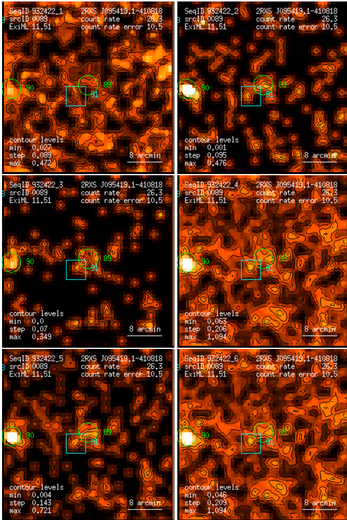
Figure 89: RASS 932422: detection 0089: band rate images, Gaussian filter: (1) PSPC channels 11 – 41, (2) 52 – 90, (3) 91 – 201, (4) 11 – 235, (5) 52 – 201, (6) 11 – 201. Broad band rates in counts/ks. Band rate contour levels in counts/ks/arcmin 2 .
