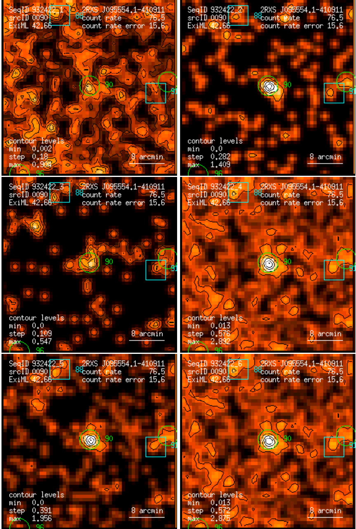
Figure 90: RASS 932422: detection 0090: band rate images, Gaussian filter: (1) PSPC channels 11 – 41, (2) 52 – 90, (3) 91 – 201, (4) 11 – 235, (5) 52 – 201, (6) 11 – 201. Broad band rates in counts/ks. Band rate contour levels in counts/ks/arcmin 2 .
