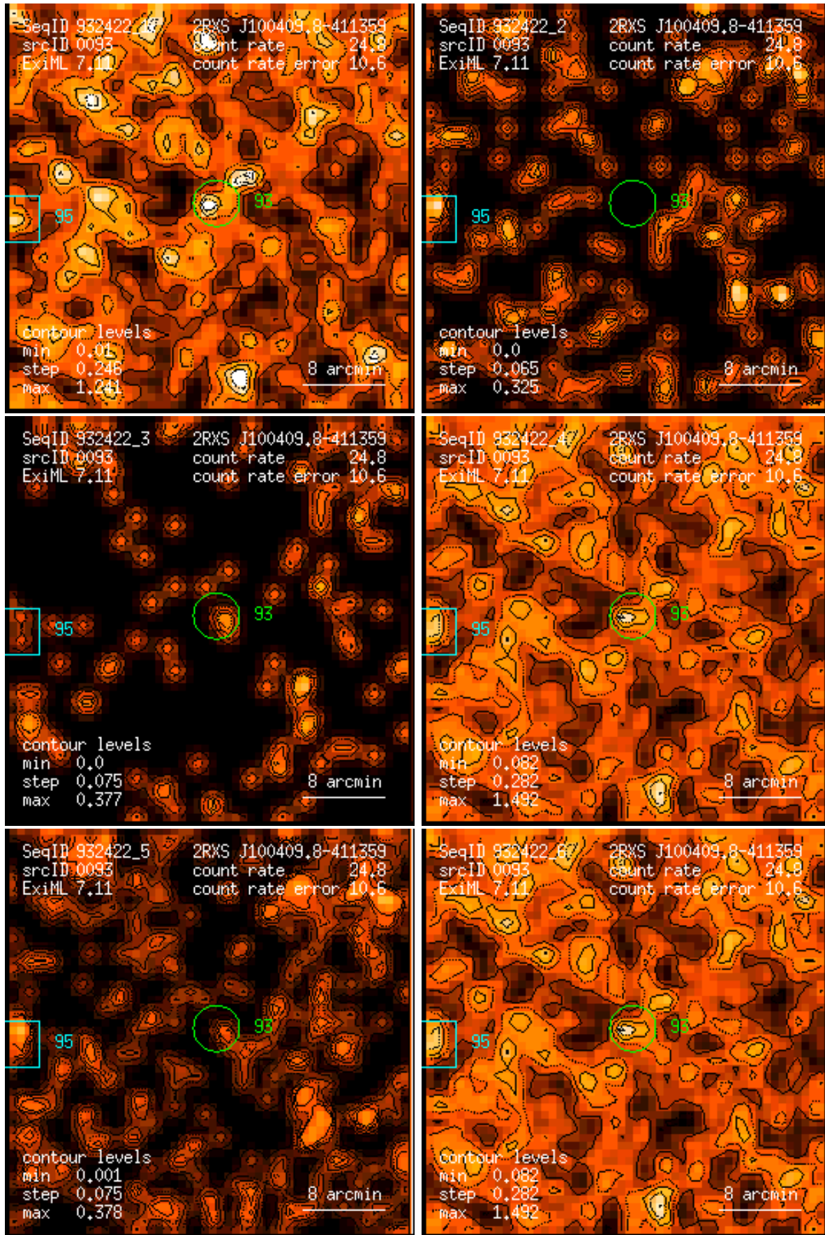
Figure 93: RASS 932422: detection 0093: band rate images, Gaussian filter: (1) PSPC channels 11 – 41, (2) 52 – 90, (3) 91 – 201, (4) 11 – 235, (5) 52 – 201, (6) 11 – 201. Broad band rates in counts/ks. Band rate contour levels in counts/ks/arcmin 2 .
