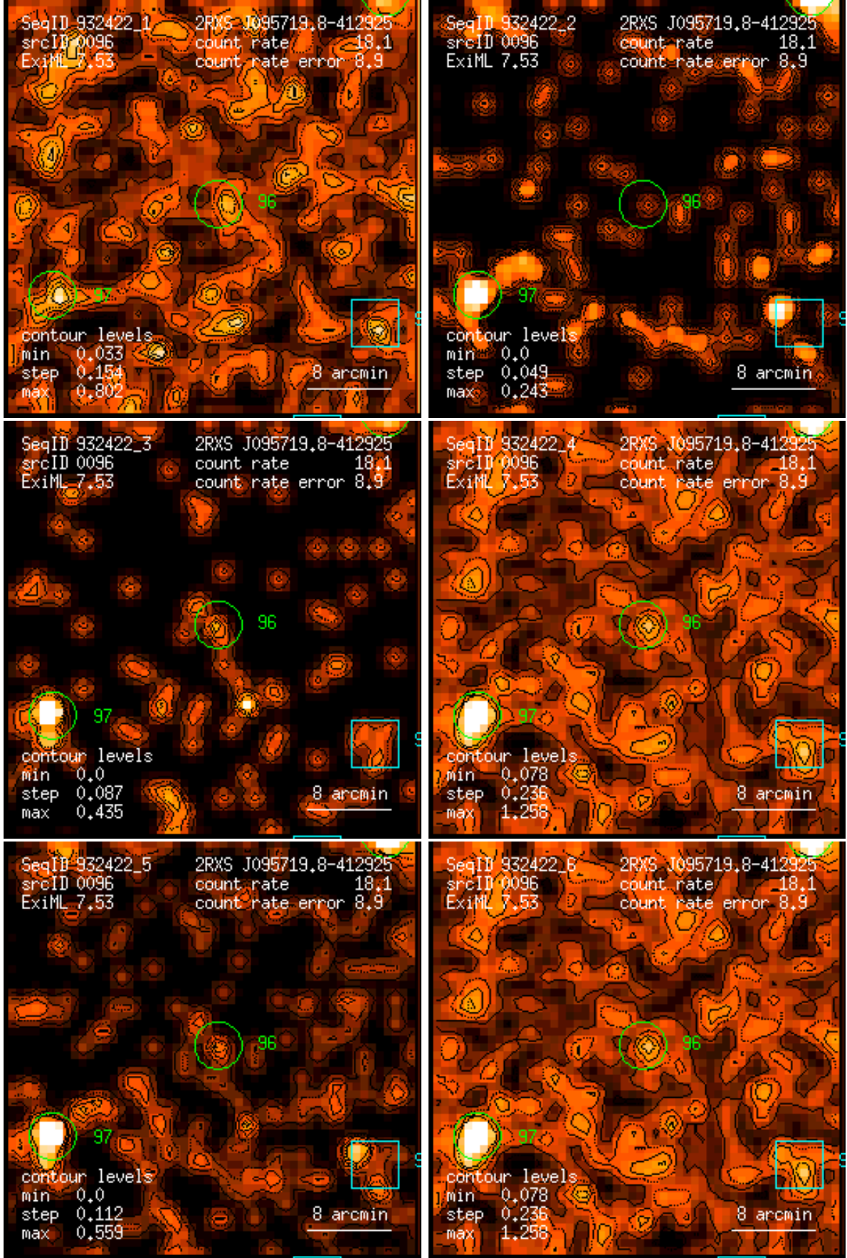
Figure 96: RASS 932422: detection 0096: band rate images, Gaussian filter: (1) PSPC channels 11 – 41, (2) 52 – 90, (3) 91 – 201, (4) 11 – 235, (5) 52 – 201, (6) 11 – 201. Broad band rates in counts/ks. Band rate contour levels in counts/ks/arcmin 2 .
