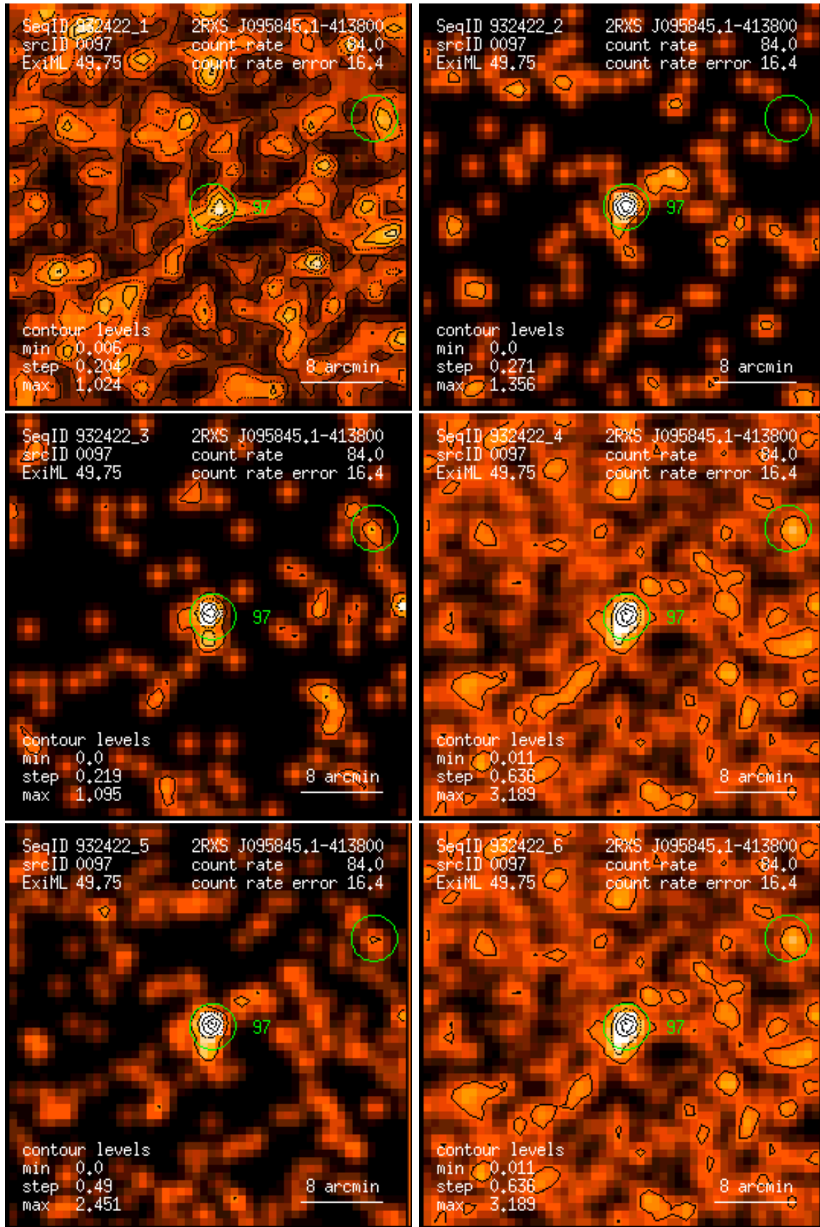
Figure 97: RASS 932422: detection 0097: band rate images, Gaussian filter: (1) PSPC channels 11 – 41, (2) 52 – 90, (3) 91 – 201, (4) 11 – 235, (5) 52 – 201, (6) 11 – 201. Broad band rates in counts/ks. Band rate contour levels in counts/ks/arcmin 2 .
