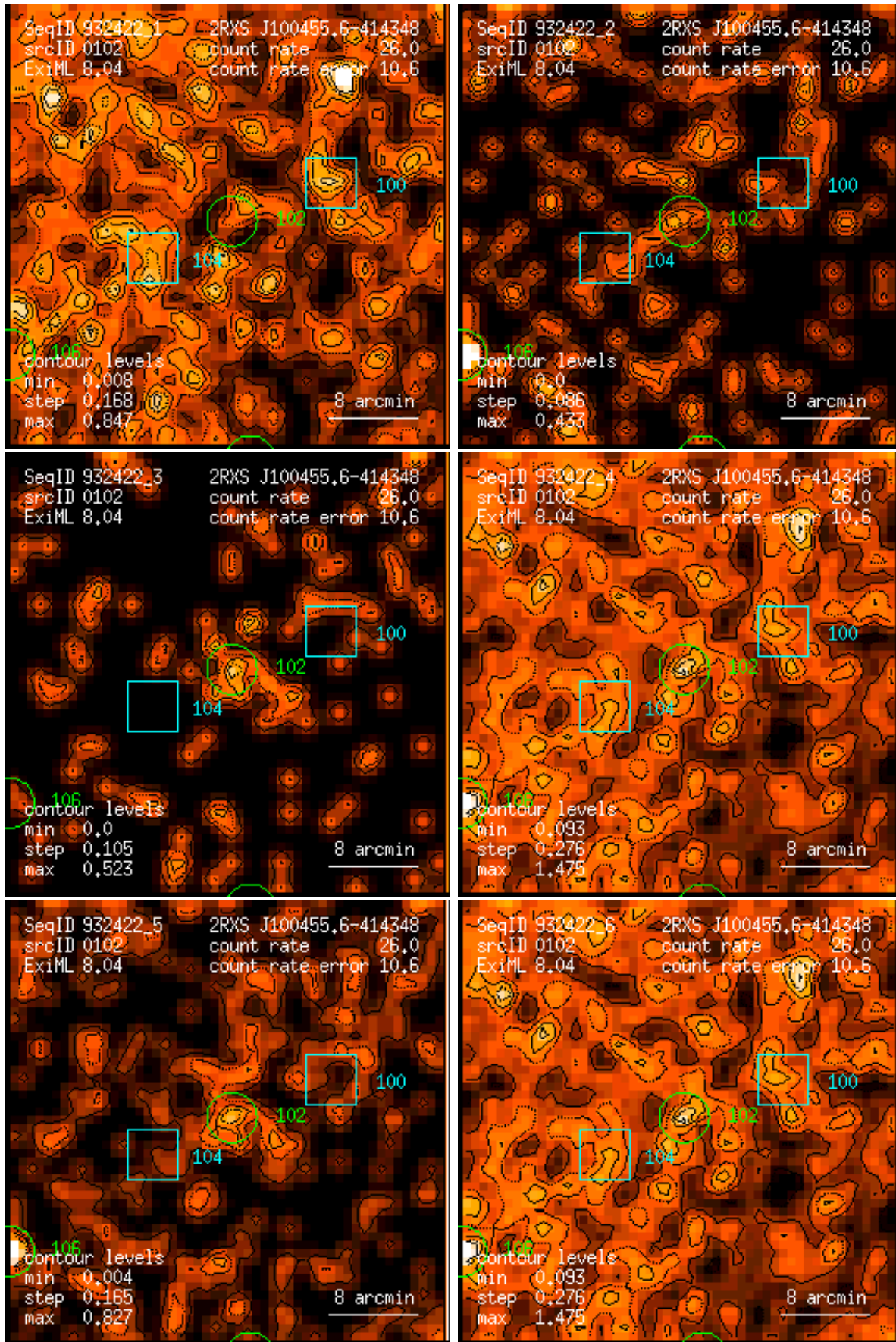
Figure 102: RASS 932422: detection 0102: band rate images, Gaussian filter: (1) PSPC channels 11 – 41, (2) 52 – 90, (3) 91 – 201, (4) 11 – 235, (5) 52 – 201, (6) 11 – 201. Broad band rates in counts/ks. Band rate contour levels in counts/ks/arcmin 2 .
