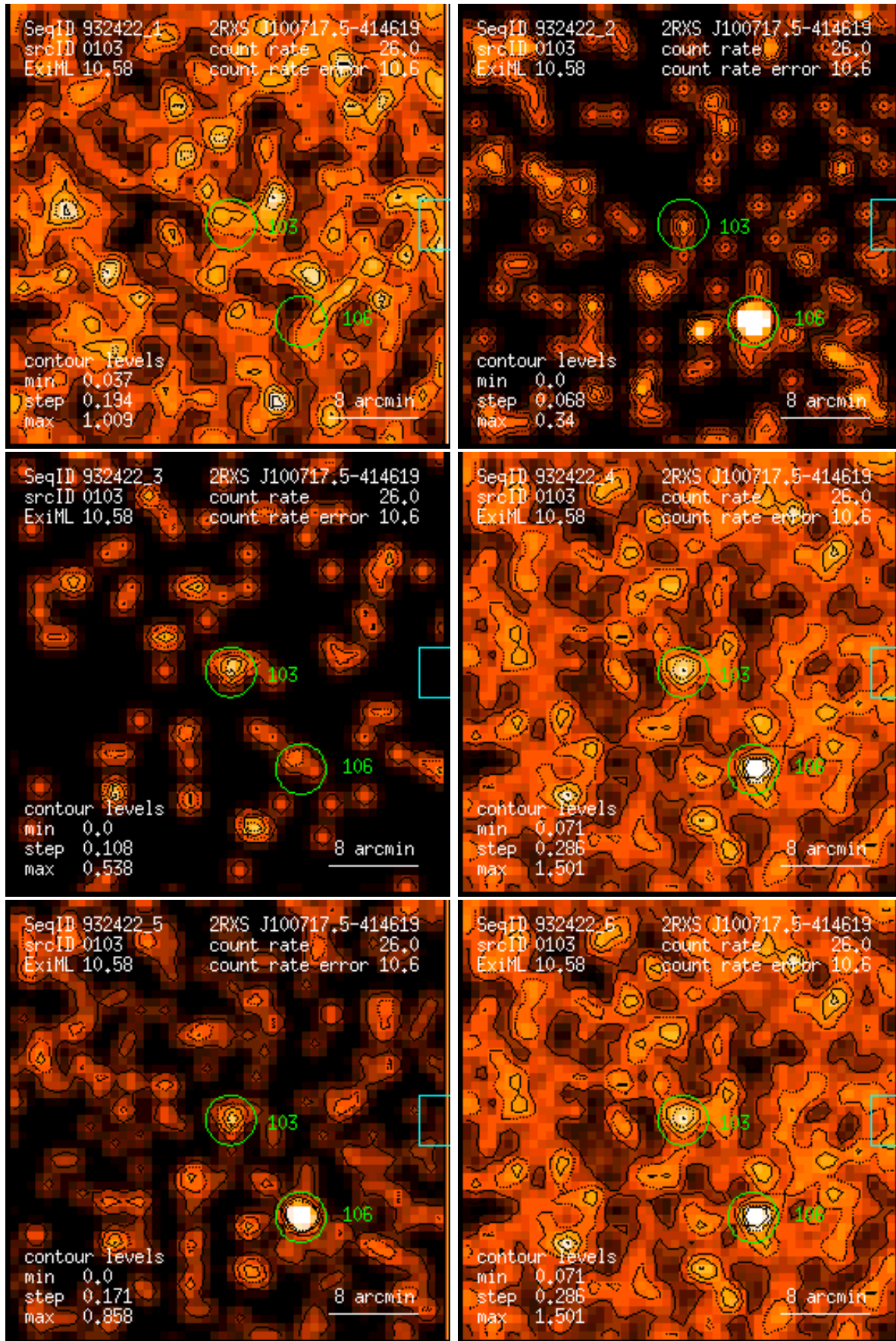
Figure 103: RASS 932422: detection 0103: band rate images, Gaussian filter: (1) PSPC channels 11 – 41, (2) 52 – 90, (3) 91 – 201, (4) 11 – 235, (5) 52 – 201, (6) 11 – 201. Broad band rates in counts/ks. Band rate contour levels in counts/ks/arcmin 2 .
