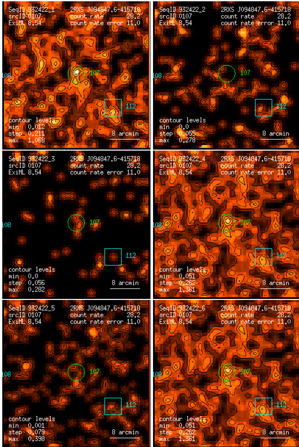
Figure 107: RASS 932422: detection 0107: band rate images, Gaussian filter: (1) PSPC channels 11 – 41, (2) 52 – 90, (3) 91 – 201, (4) 11 – 235, (5) 52 – 201, (6) 11 – 201. Broad band rates in counts/ks. Band rate contour levels in counts/ks/arcmin 2 .
