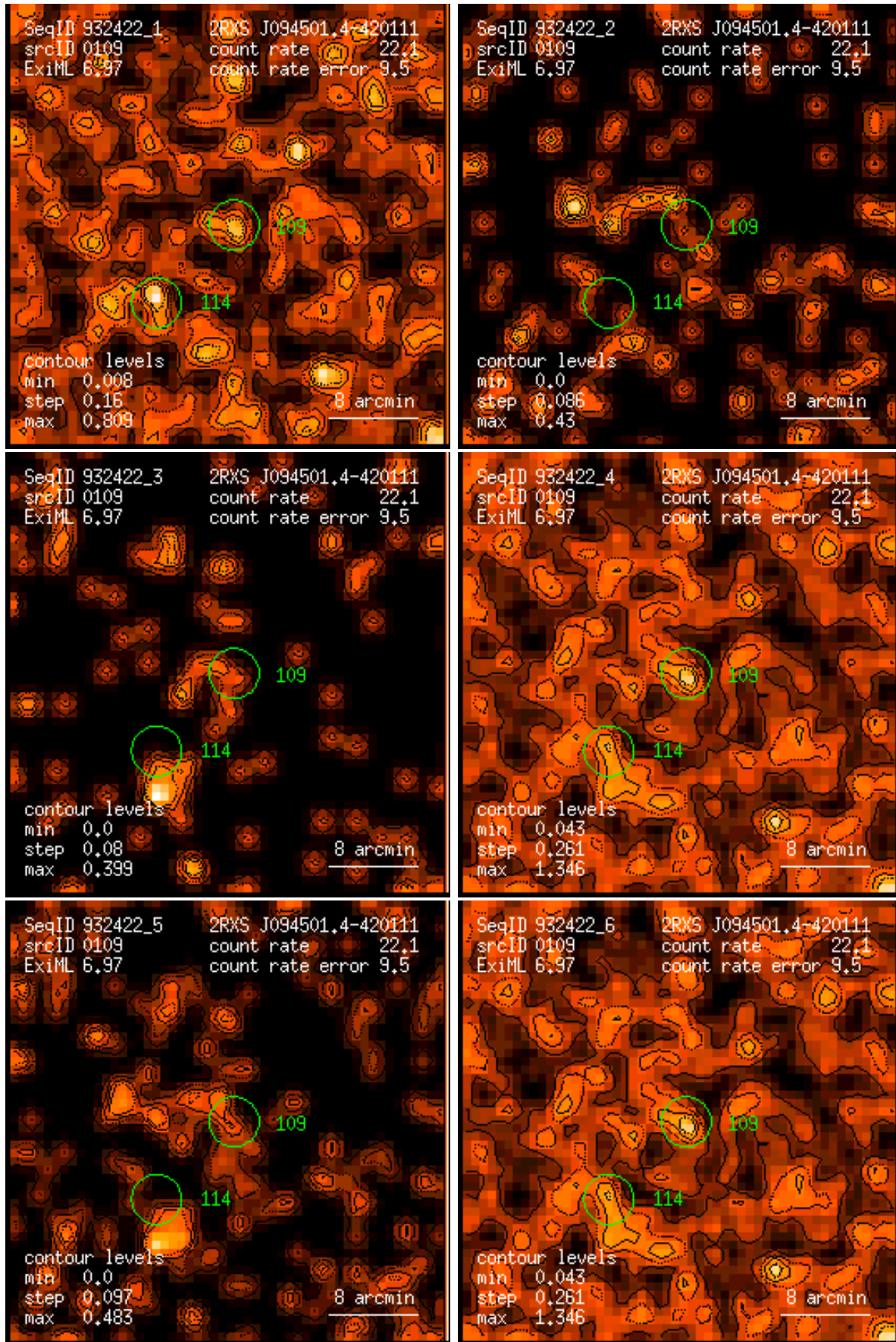
Figure 109: RASS 932422: detection 0109: band rate images, Gaussian filter: (1) PSPC channels 11 – 41, (2) 52 – 90, (3) 91 – 201, (4) 11 – 235, (5) 52 – 201, (6) 11 – 201. Broad band rates in counts/ks. Band rate contour levels in counts/ks/arcmin 2 .
